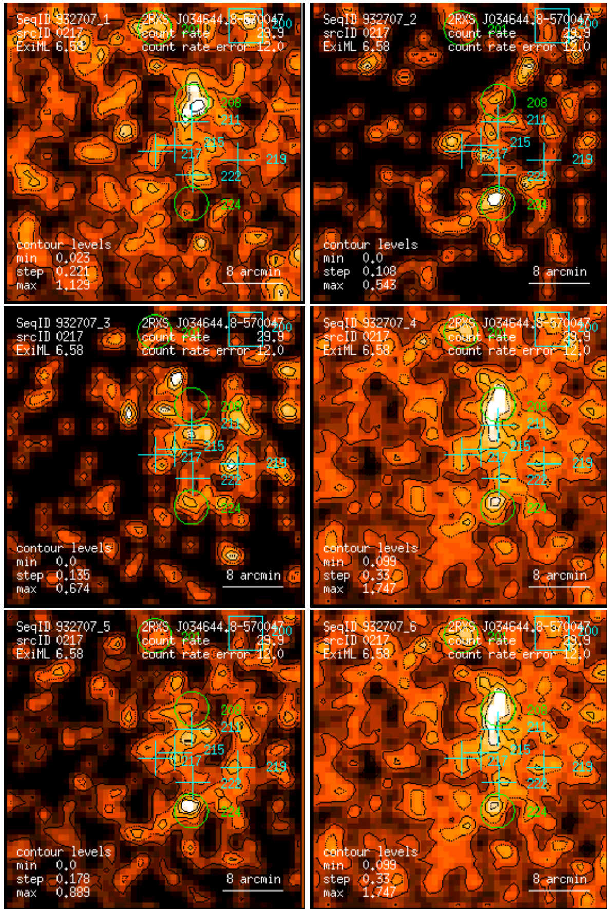
Figure 217: RASS 932707: detection 0217: band rate images, Gaussian filter: (1) PSPC channels 11 – 41, (2) 52 – 90, (3) 91 – 201, (4) 11 – 235, (5) 52 – 201, (6) 11 – 201. Broad band rates in counts/ks. Band rate contour levels in counts/ks/arcmin 2 .
