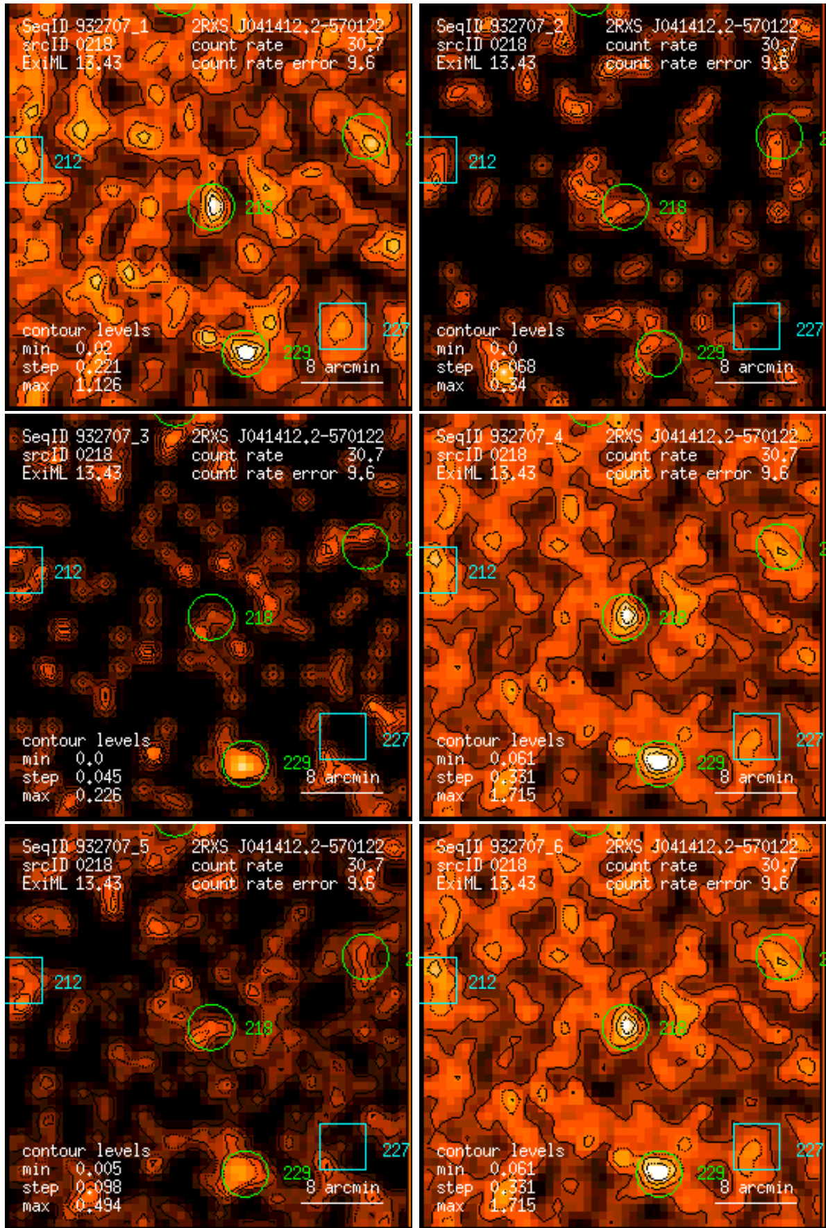
Figure 218: RASS 932707: detection 0218: band rate images, Gaussian filter: (1) PSPC channels 11 – 41, (2) 52 – 90, (3) 91 – 201, (4) 11 – 235, (5) 52 – 201, (6) 11 – 201. Broad band rates in counts/ks. Band rate contour levels in counts/ks/arcmin 2 .
