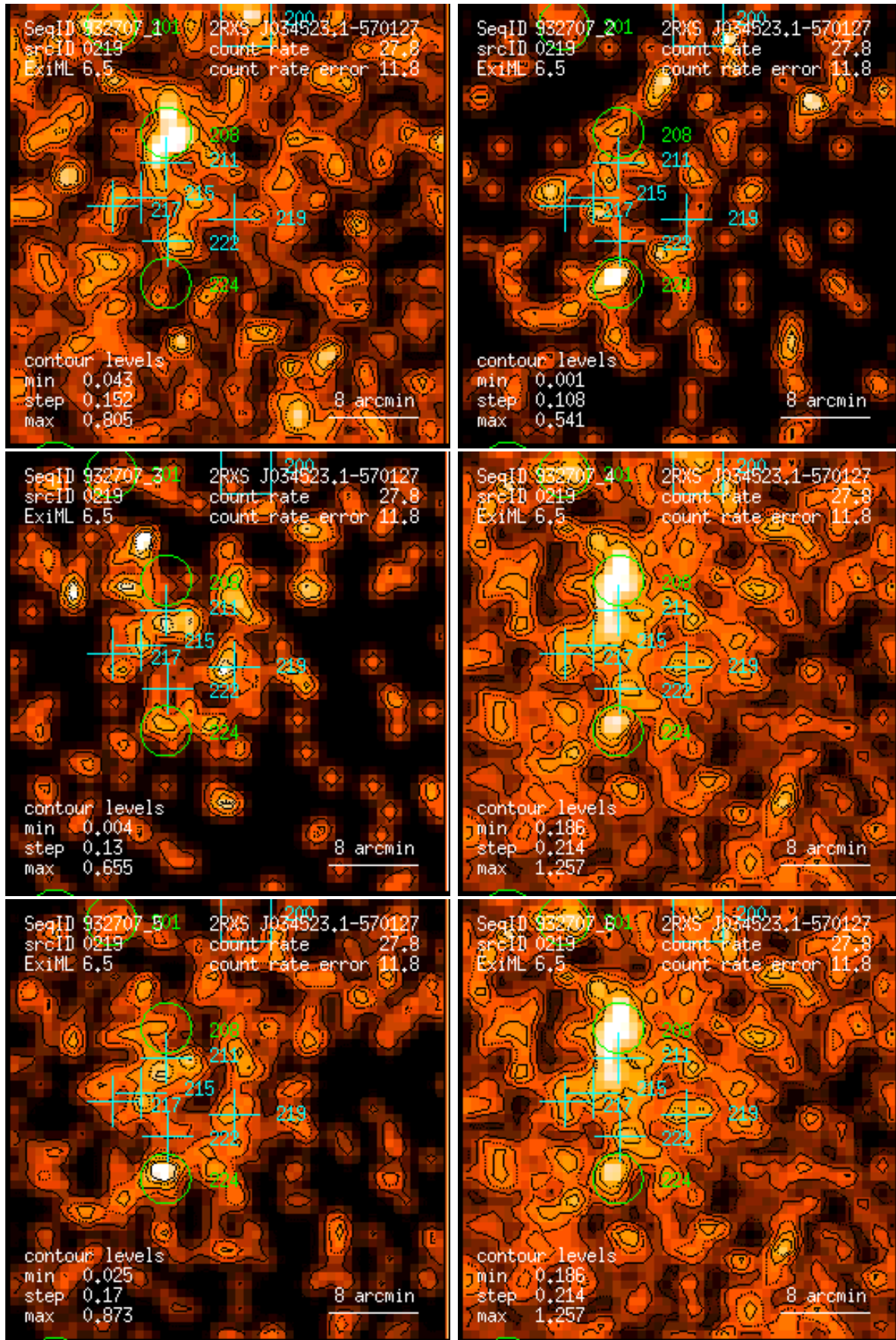
Figure 219: RASS 932707: detection 0219: band rate images, Gaussian filter: (1) PSPC channels 11 – 41, (2) 52 – 90, (3) 91 – 201, (4) 11 – 235, (5) 52 – 201, (6) 11 – 201. Broad band rates in counts/ks. Band rate contour levels in counts/ks/arcmin 2 .
