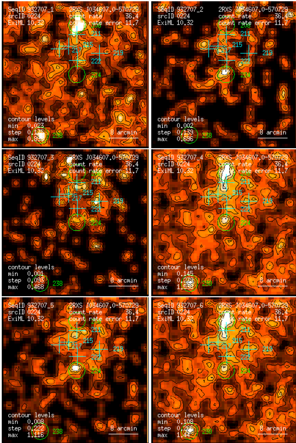
Figure 224: RASS 932707: detection 0224: band rate images, Gaussian filter: (1) PSPC channels 11 – 41, (2) 52 – 90, (3) 91 – 201, (4) 11 – 235, (5) 52 – 201, (6) 11 – 201. Broad band rates in counts/ks. Band rate contour levels in counts/ks/arcmin 2 .
