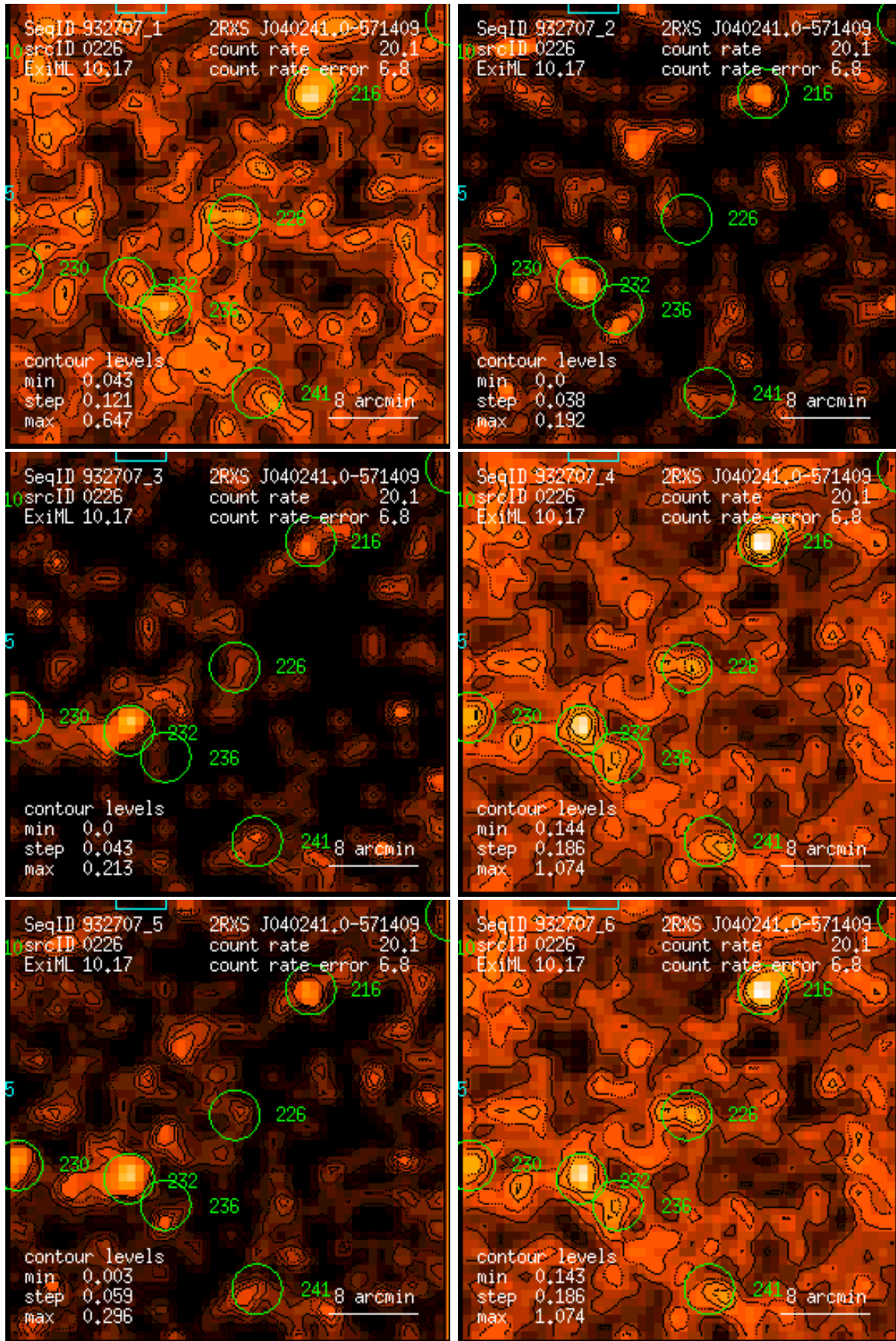
Figure 226: RASS 932707: detection 0226: band rate images, Gaussian filter: (1) PSPC channels 11 – 41, (2) 52 – 90, (3) 91 – 201, (4) 11 – 235, (5) 52 – 201, (6) 11 – 201. Broad band rates in counts/ks. Band rate contour levels in counts/ks/arcmin 2 .
