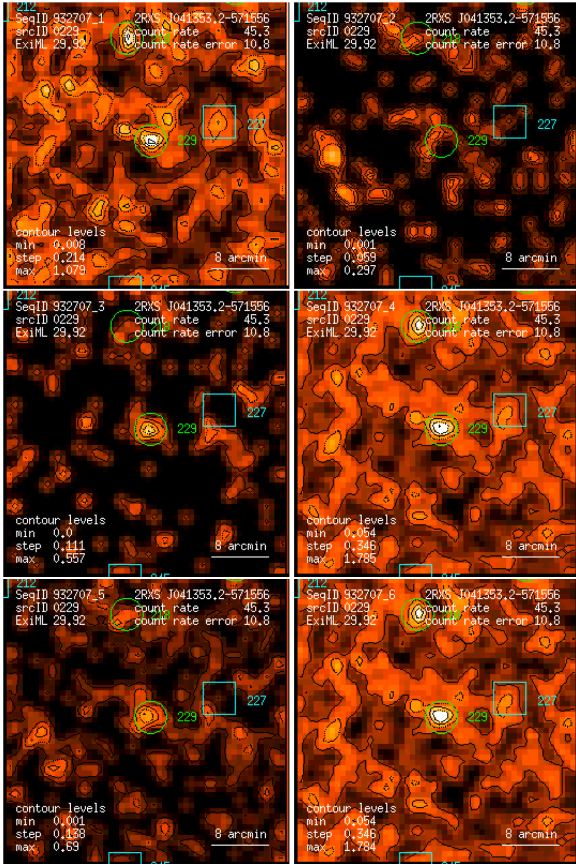
Figure 229: RASS 932707: detection 0229: band rate images, Gaussian filter: (1) PSPC channels 11 – 41, (2) 52 – 90, (3) 91 – 201, (4) 11 – 235, (5) 52 – 201, (6) 11 – 201. Broad band rates in counts/ks. Band rate contour levels in counts/ks/arcmin 2 .
