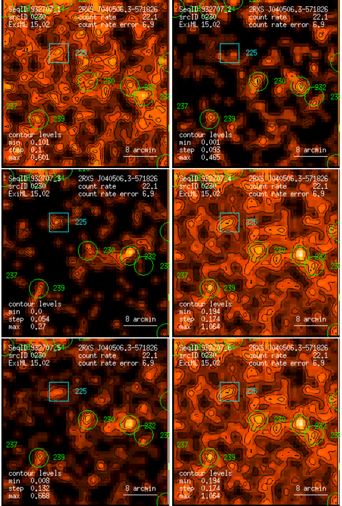
Figure 230: RASS 932707: detection 0230: band rate images, Gaussian filter: (1) PSPC channels 11 – 41, (2) 52 – 90, (3) 91 – 201, (4) 11 – 235, (5) 52 – 201, (6) 11 – 201. Broad band rates in counts/ks. Band rate contour levels in counts/ks/arcmin 2 .
