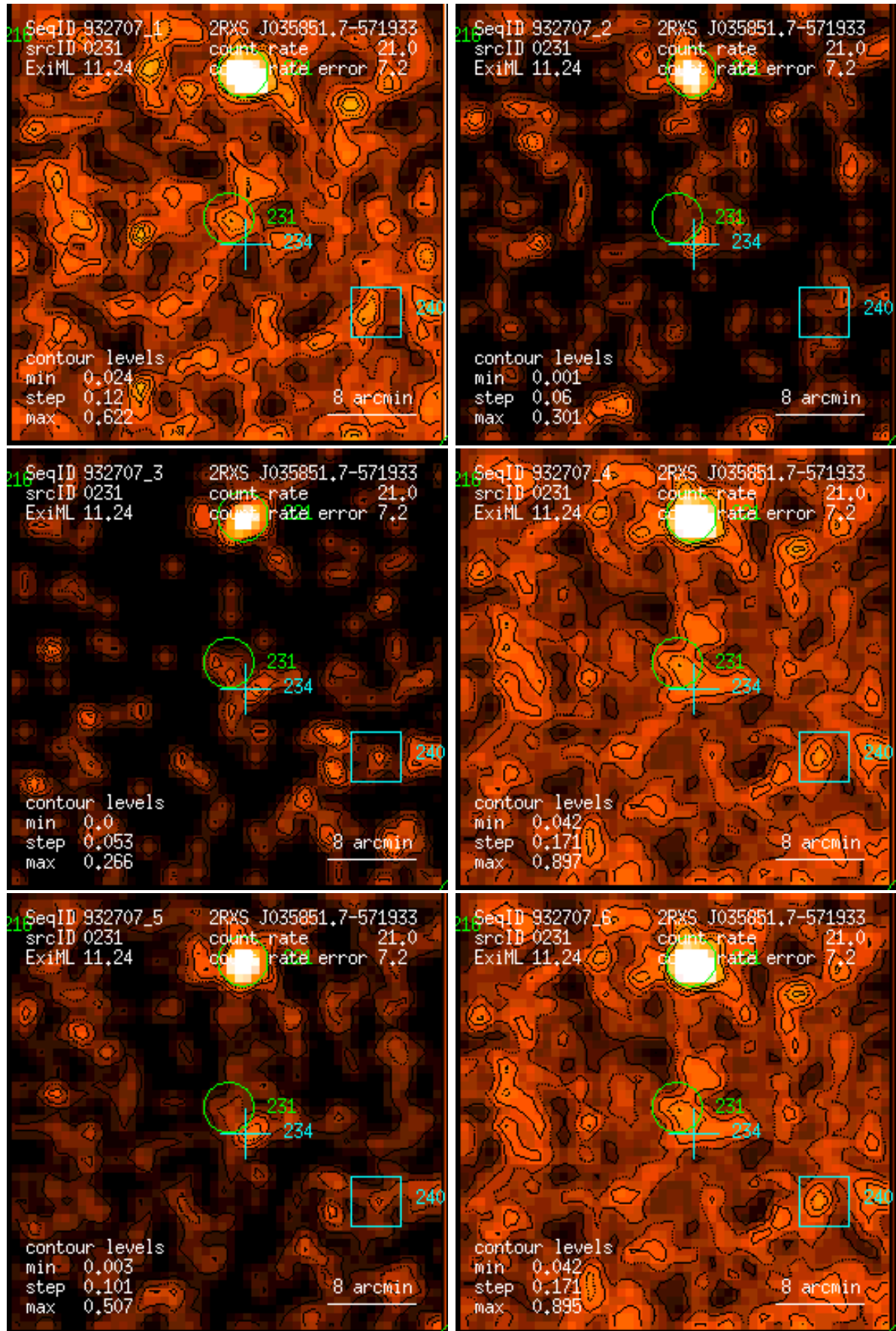
Figure 231: RASS 932707: detection 0231: band rate images, Gaussian filter: (1) PSPC channels 11 – 41, (2) 52 – 90, (3) 91 – 201, (4) 11 – 235, (5) 52 – 201, (6) 11 – 201. Broad band rates in counts/ks. Band rate contour levels in counts/ks/arcmin 2 .
