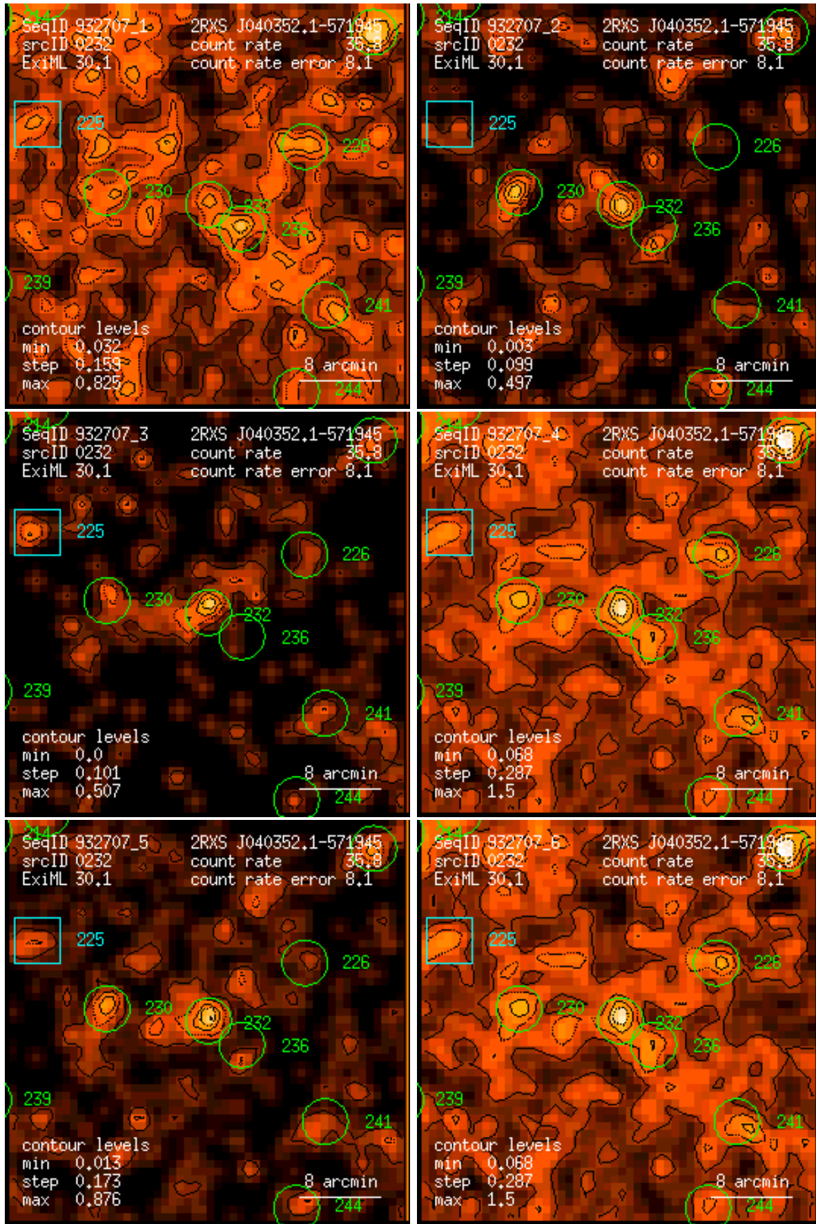
Figure 232: RASS 932707: detection 0232: band rate images, Gaussian filter: (1) PSPC channels 11 – 41, (2) 52 – 90, (3) 91 – 201, (4) 11 – 235, (5) 52 – 201, (6) 11 – 201. Broad band rates in counts/ks. Band rate contour levels in counts/ks/arcmin 2 .
