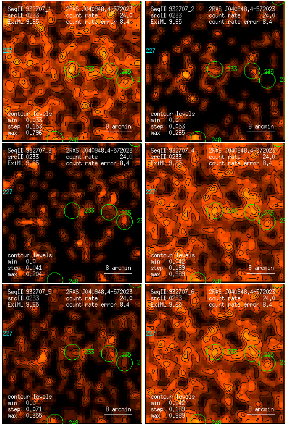
Figure 233: RASS 932707: detection 0233: band rate images, Gaussian filter: (1) PSPC channels 11 – 41, (2) 52 – 90, (3) 91 – 201, (4) 11 – 235, (5) 52 – 201, (6) 11 – 201. Broad band rates in counts/ks. Band rate contour levels in counts/ks/arcmin 2 .
