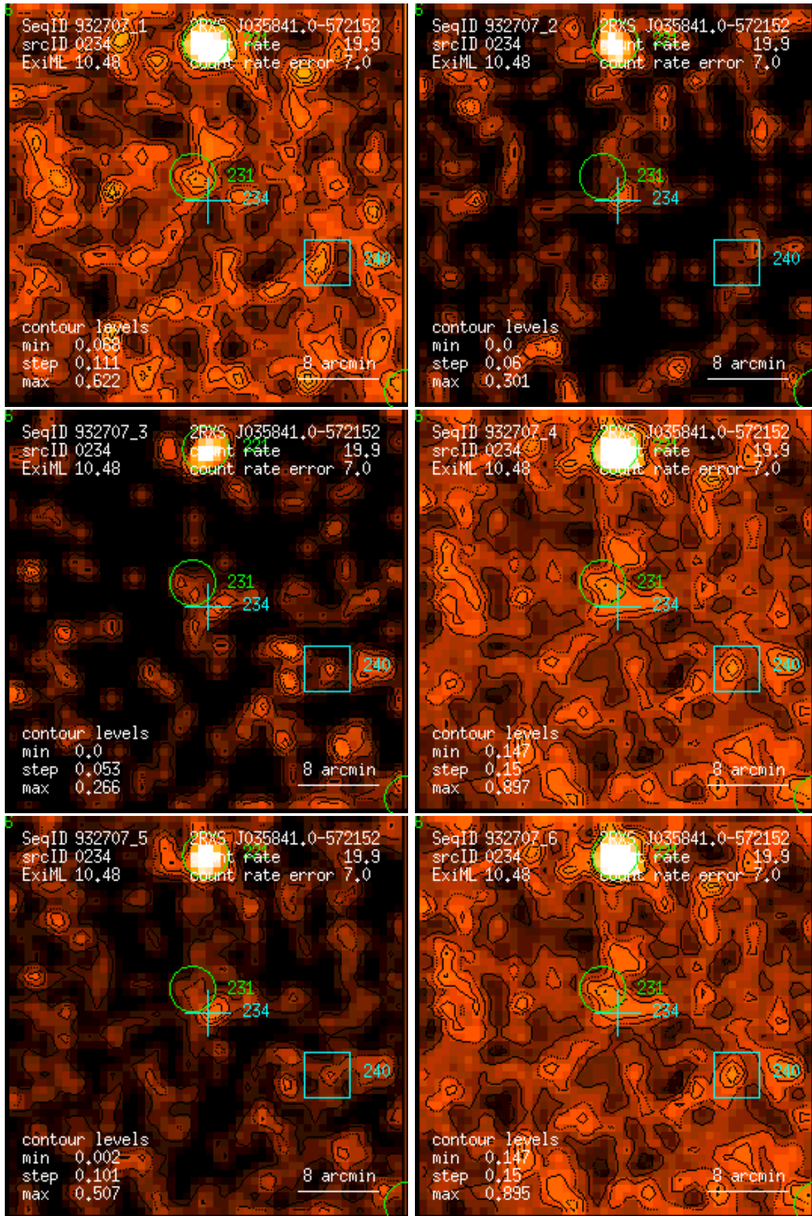
Figure 234: RASS 932707: detection 0234: band rate images, Gaussian filter: (1) PSPC channels 11 – 41, (2) 52 – 90, (3) 91 – 201, (4) 11 – 235, (5) 52 – 201, (6) 11 – 201. Broad band rates in counts/ks. Band rate contour levels in counts/ks/arcmin 2 .
