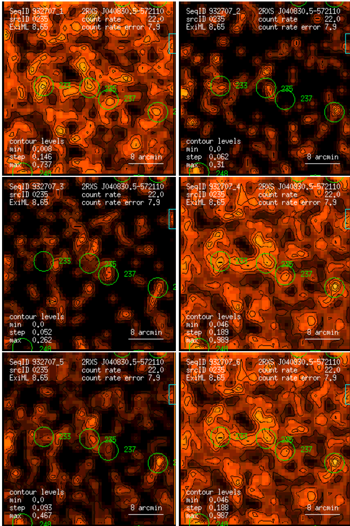
Figure 235: RASS 932707: detection 0235: band rate images, Gaussian filter: (1) PSPC channels 11 – 41, (2) 52 – 90, (3) 91 – 201, (4) 11 – 235, (5) 52 – 201, (6) 11 – 201. Broad band rates in counts/ks. Band rate contour levels in counts/ks/arcmin 2 .
