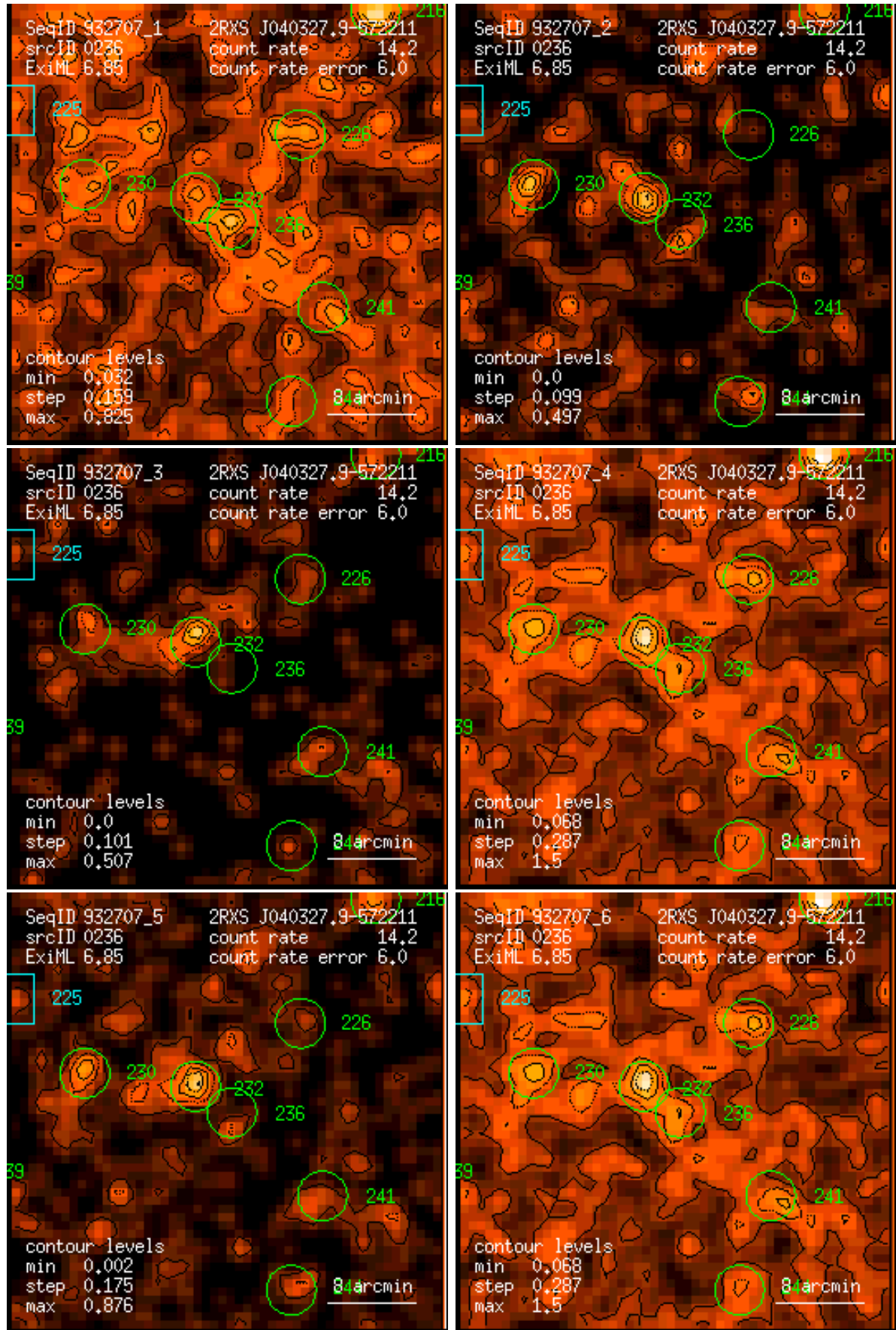
Figure 236: RASS 932707: detection 0236: band rate images, Gaussian filter: (1) PSPC channels 11 – 41, (2) 52 – 90, (3) 91 – 201, (4) 11 – 235, (5) 52 – 201, (6) 11 – 201. Broad band rates in counts/ks. Band rate contour levels in counts/ks/arcmin 2 .
