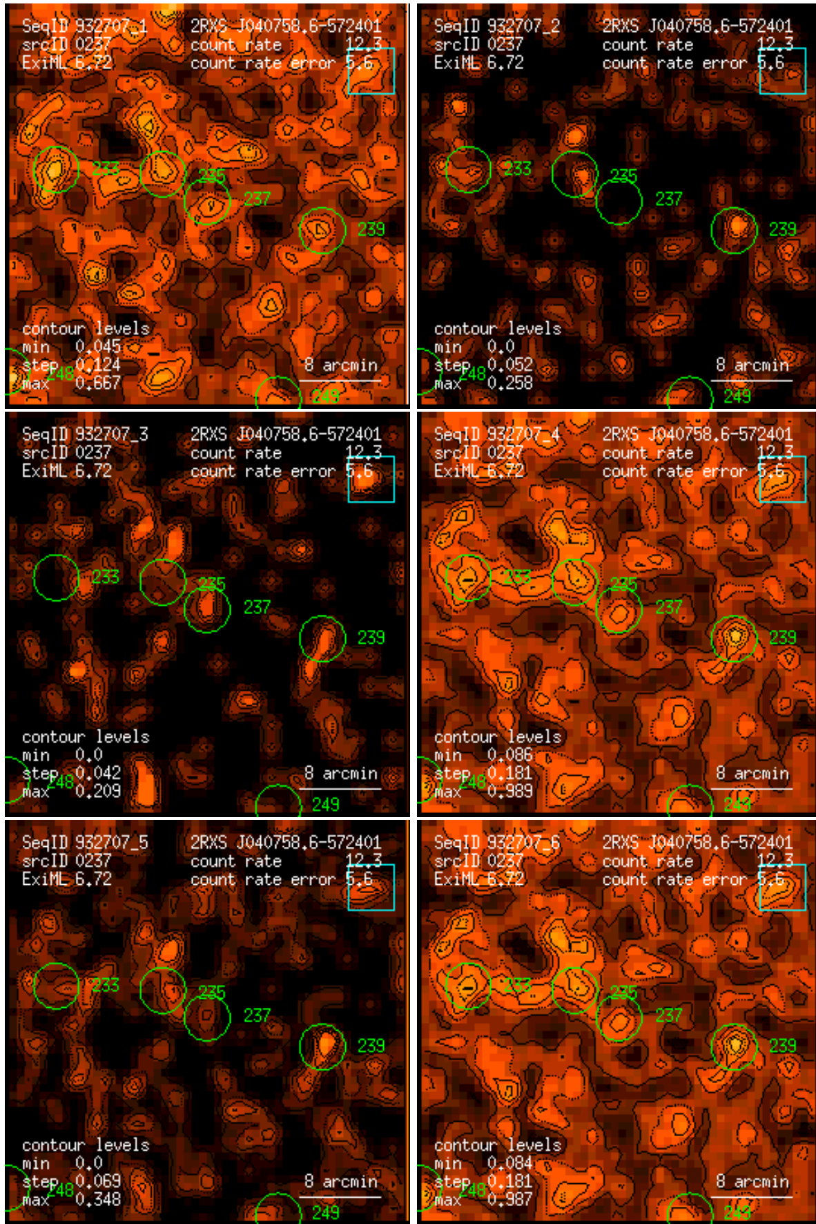
Figure 237: RASS 932707: detection 0237: band rate images, Gaussian filter: (1) PSPC channels 11 – 41, (2) 52 – 90, (3) 91 – 201, (4) 11 – 235, (5) 52 – 201, (6) 11 – 201. Broad band rates in counts/ks. Band rate contour levels in counts/ks/arcmin 2 .
