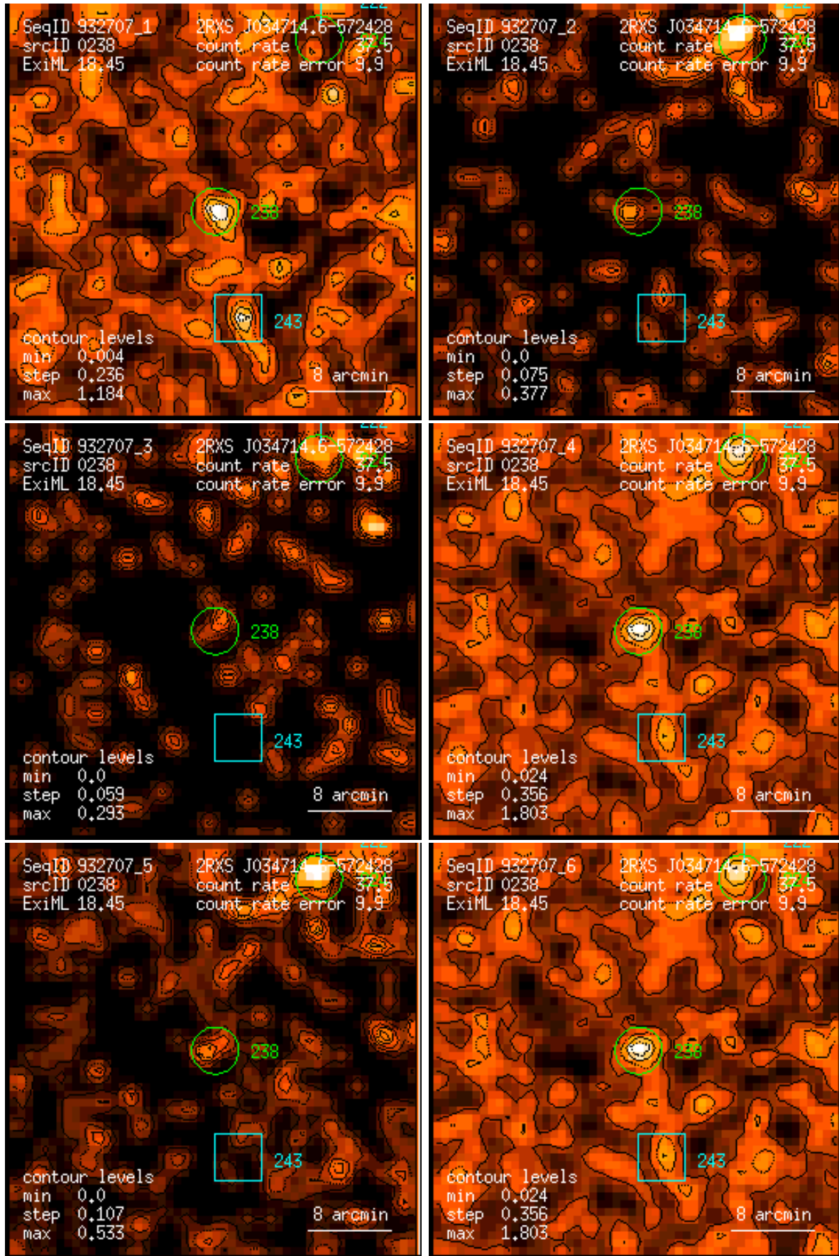
Figure 238: RASS 932707: detection 0238: band rate images, Gaussian filter: (1) PSPC channels 11 – 41, (2) 52 – 90, (3) 91 – 201, (4) 11 – 235, (5) 52 – 201, (6) 11 – 201. Broad band rates in counts/ks. Band rate contour levels in counts/ks/arcmin 2 .
