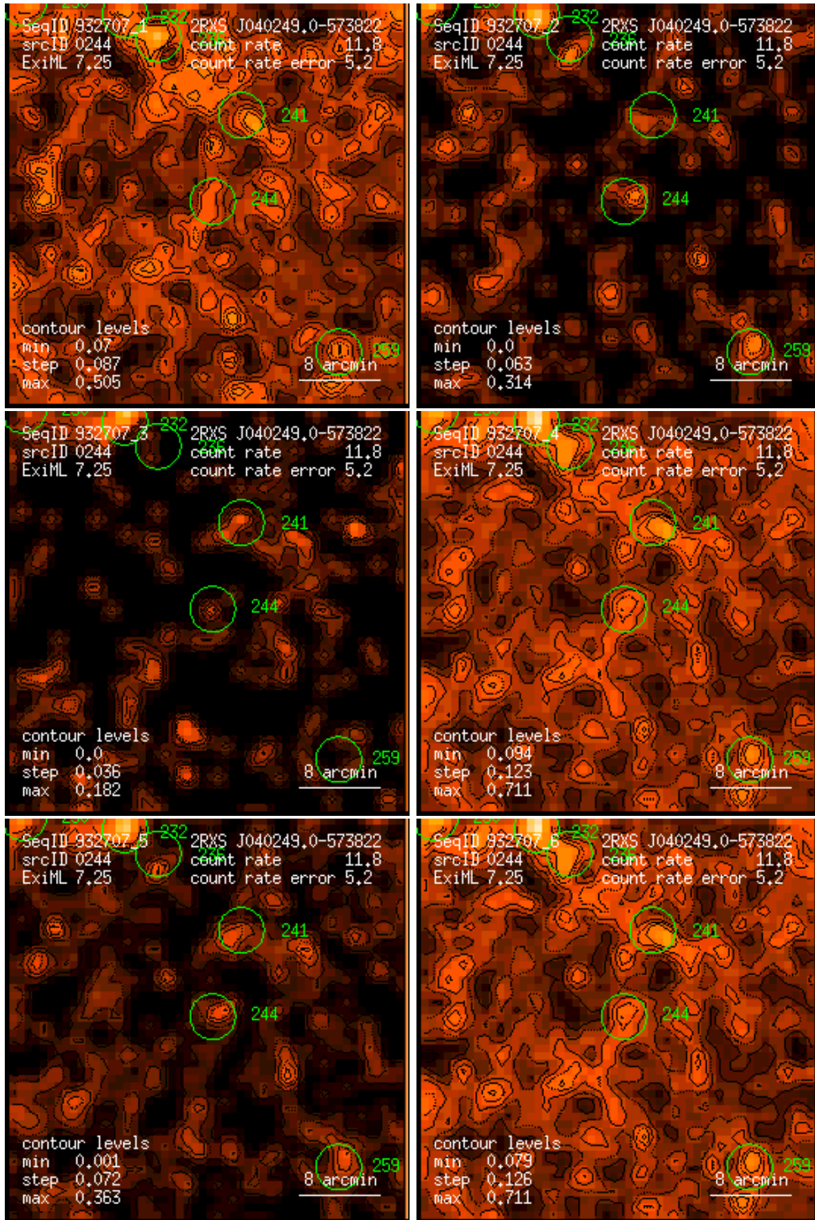
Figure 244: RASS 932707: detection 0244: band rate images, Gaussian filter: (1) PSPC channels 11 – 41, (2) 52 – 90, (3) 91 – 201, (4) 11 – 235, (5) 52 – 201, (6) 11 – 201. Broad band rates in counts/ks. Band rate contour levels in counts/ks/arcmin 2 .
