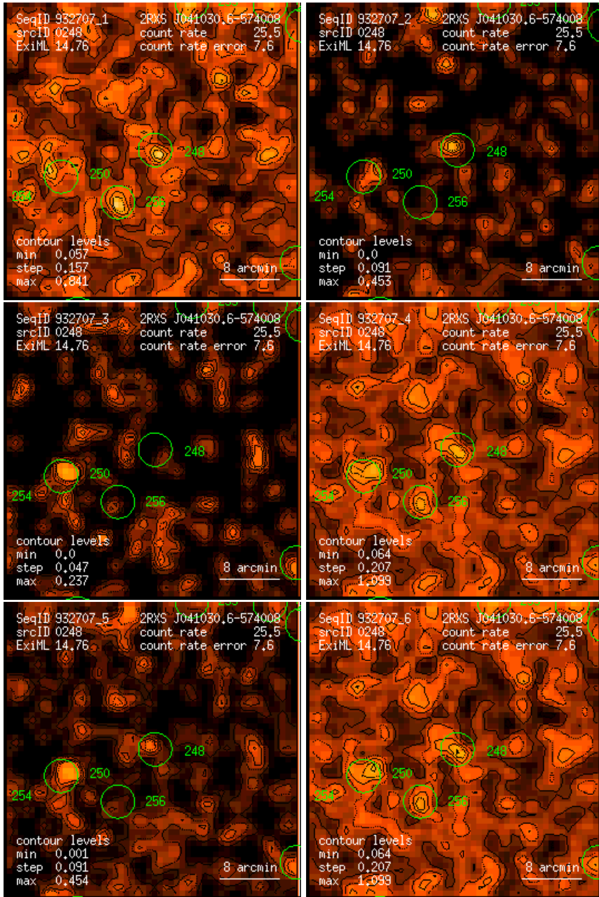
Figure 248: RASS 932707: detection 0248: band rate images, Gaussian filter: (1) PSPC channels 11 – 41, (2) 52 – 90, (3) 91 – 201, (4) 11 – 235, (5) 52 – 201, (6) 11 – 201. Broad band rates in counts/ks. Band rate contour levels in counts/ks/arcmin 2 .
