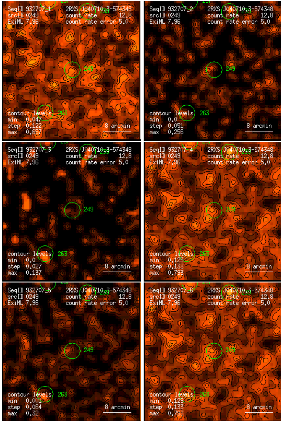
Figure 249: RASS 932707: detection 0249: band rate images, Gaussian filter: (1) PSPC channels 11 – 41, (2) 52 – 90, (3) 91 – 201, (4) 11 – 235, (5) 52 – 201, (6) 11 – 201. Broad band rates in counts/ks. Band rate contour levels in counts/ks/arcmin 2 .
