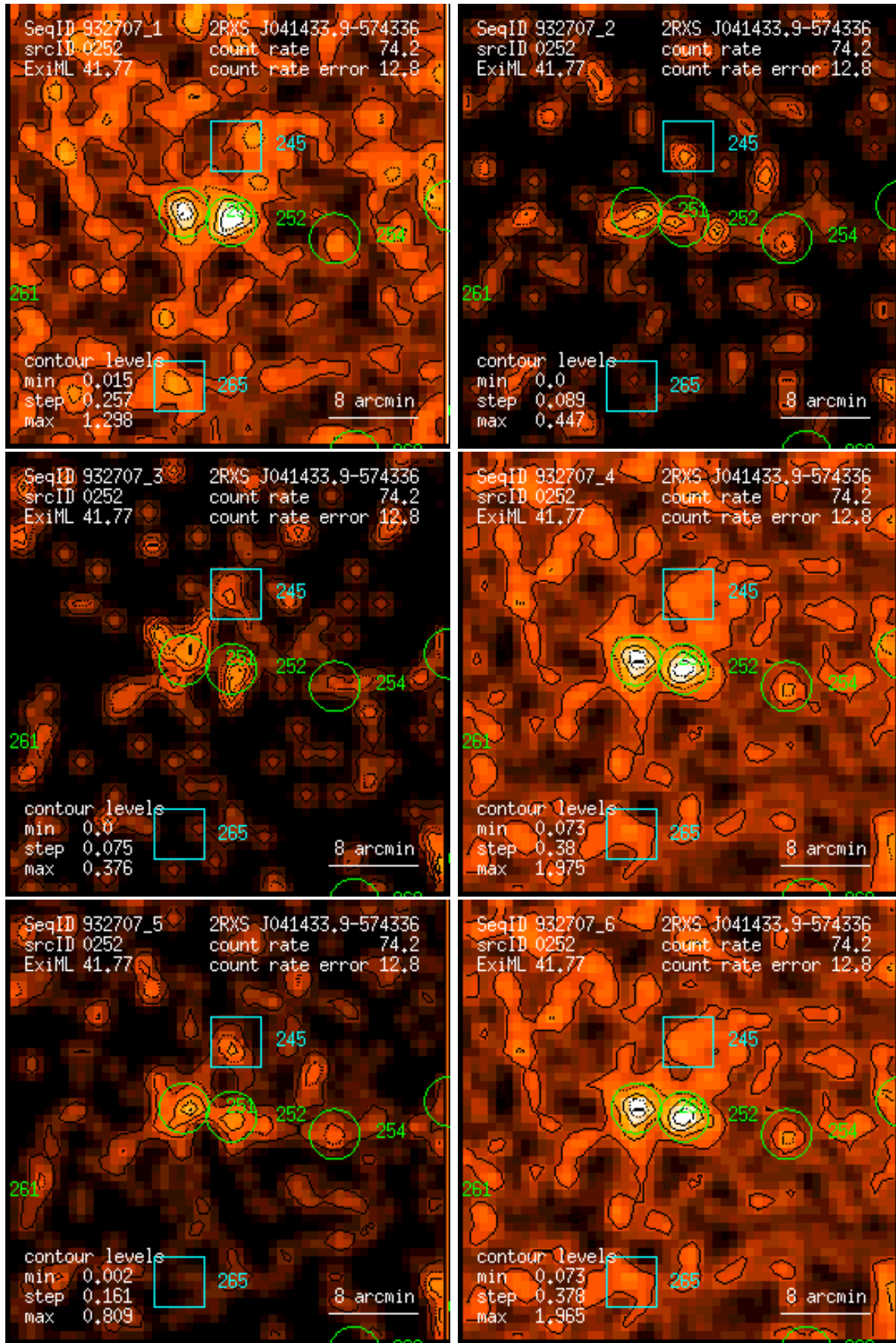
Figure 252: RASS 932707: detection 0252: band rate images, Gaussian filter: (1) PSPC channels 11 – 41, (2) 52 – 90, (3) 91 – 201, (4) 11 – 235, (5) 52 – 201, (6) 11 – 201. Broad band rates in counts/ks. Band rate contour levels in counts/ks/arcmin 2 .
