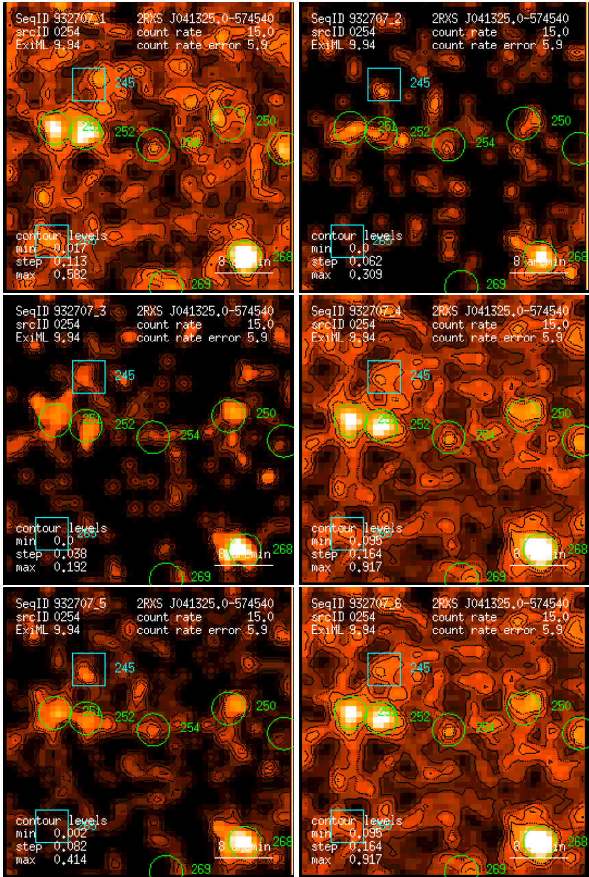
Figure 254: RASS 932707: detection 0254: band rate images, Gaussian filter: (1) PSPC channels 11 – 41, (2) 52 – 90, (3) 91 – 201, (4) 11 – 235, (5) 52 – 201, (6) 11 – 201. Broad band rates in counts/ks. Band rate contour levels in counts/ks/arcmin 2 .
