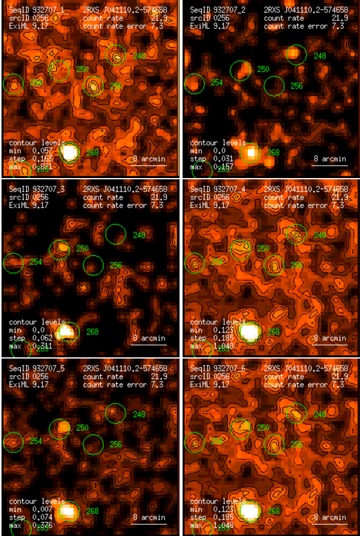
Figure 256: RASS 932707: detection 0256: band rate images, Gaussian filter: (1) PSPC channels 11 – 41, (2) 52 – 90, (3) 91 – 201, (4) 11 – 235, (5) 52 – 201, (6) 11 – 201. Broad band rates in counts/ks. Band rate contour levels in counts/ks/arcmin 2 .
