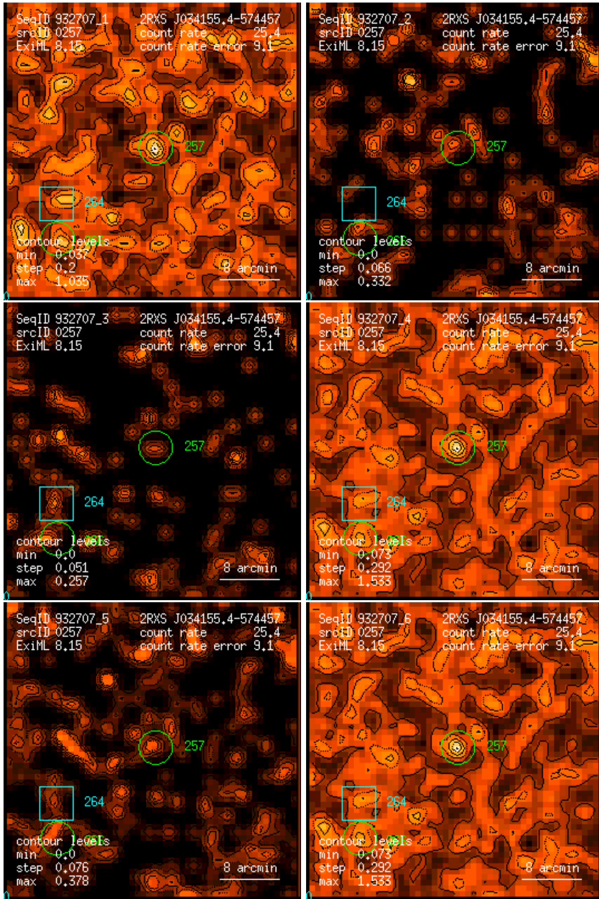
Figure 257: RASS 932707: detection 0257: band rate images, Gaussian filter: (1) PSPC channels 11 – 41, (2) 52 – 90, (3) 91 – 201, (4) 11 – 235, (5) 52 – 201, (6) 11 – 201. Broad band rates in counts/ks. Band rate contour levels in counts/ks/arcmin 2 .
