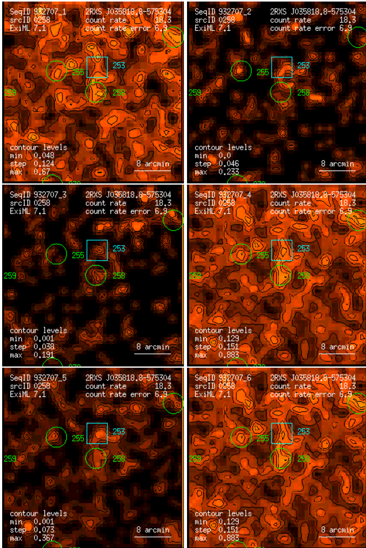
Figure 258: RASS 932707: detection 0258: band rate images, Gaussian filter: (1) PSPC channels 11 – 41, (2) 52 – 90, (3) 91 – 201, (4) 11 – 235, (5) 52 – 201, (6) 11 – 201. Broad band rates in counts/ks. Band rate contour levels in counts/ks/arcmin 2 .
