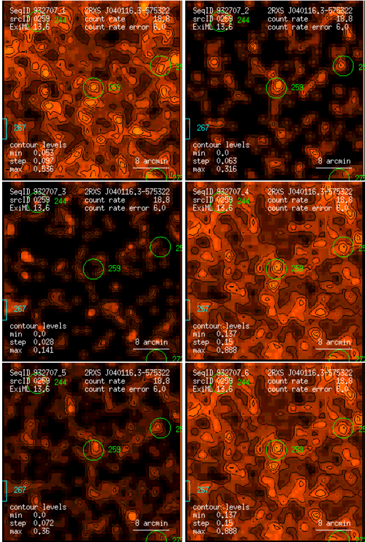
Figure 259: RASS 932707: detection 0259: band rate images, Gaussian filter: (1) PSPC channels 11 – 41, (2) 52 – 90, (3) 91 – 201, (4) 11 – 235, (5) 52 – 201, (6) 11 – 201. Broad band rates in counts/ks. Band rate contour levels in counts/ks/arcmin 2 .
