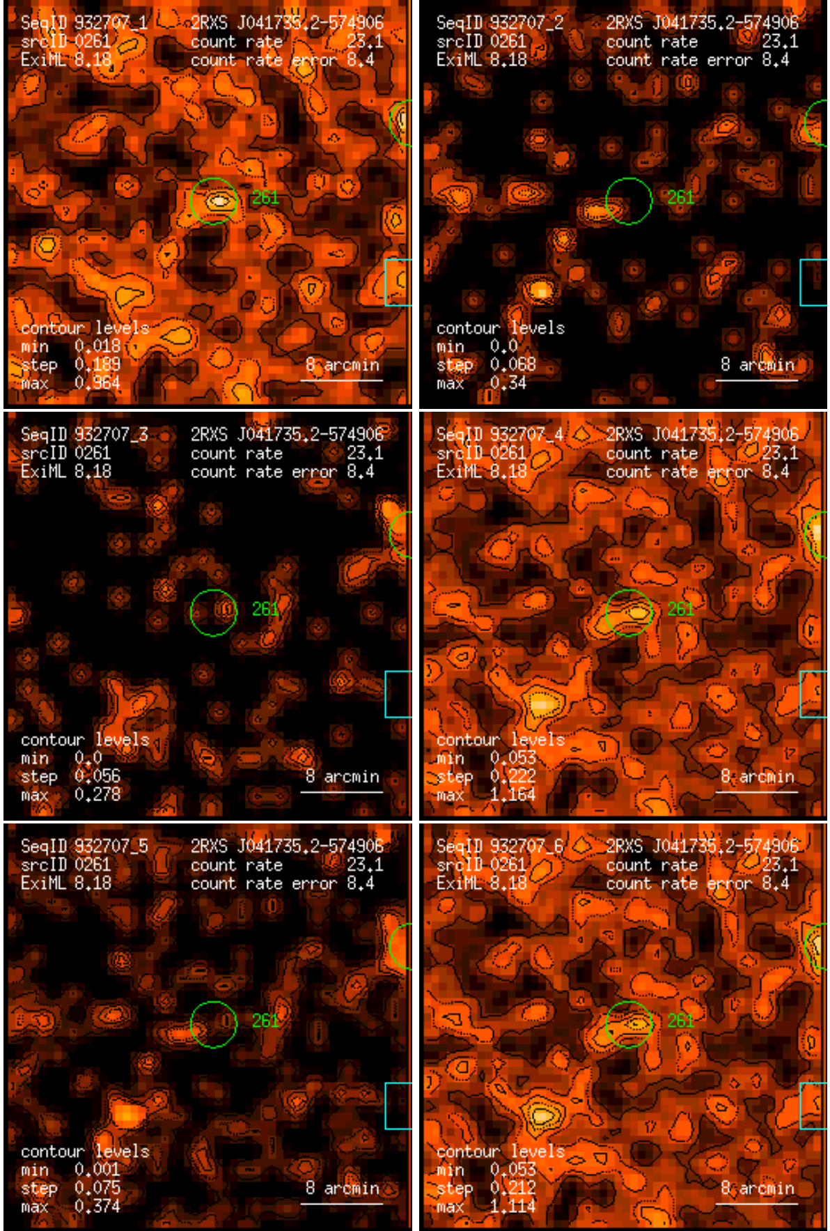
Figure 261: RASS 932707: detection 0261: band rate images, Gaussian filter: (1) PSPC channels 11 – 41, (2) 52 – 90, (3) 91 – 201, (4) 11 – 235, (5) 52 – 201, (6) 11 – 201. Broad band rates in counts/ks. Band rate contour levels in counts/ks/arcmin 2 .
