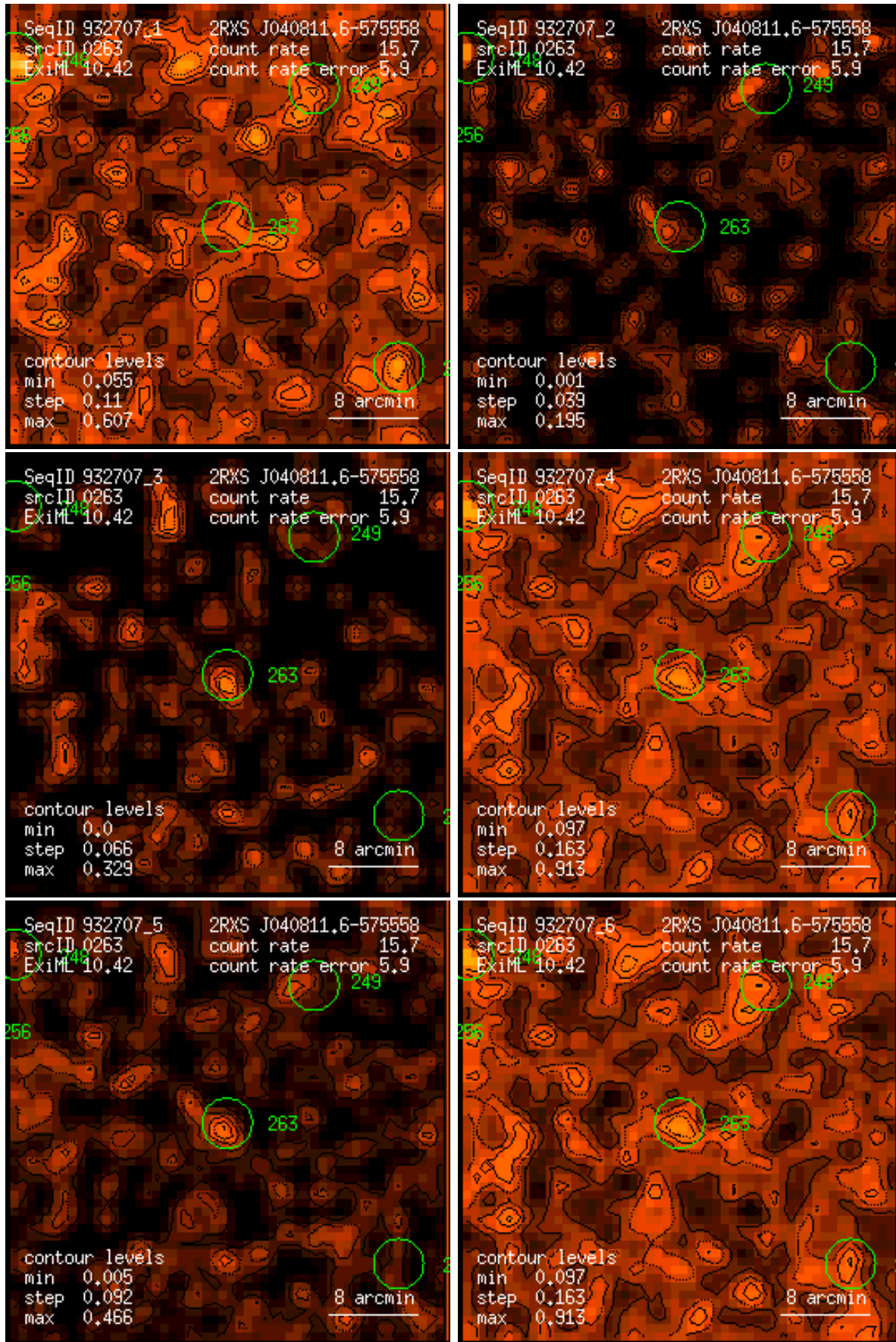
Figure 263: RASS 932707: detection 0263: band rate images, Gaussian filter: (1) PSPC channels 11 – 41, (2) 52 – 90, (3) 91 – 201, (4) 11 – 235, (5) 52 – 201, (6) 11 – 201. Broad band rates in counts/ks. Band rate contour levels in counts/ks/arcmin 2 .
