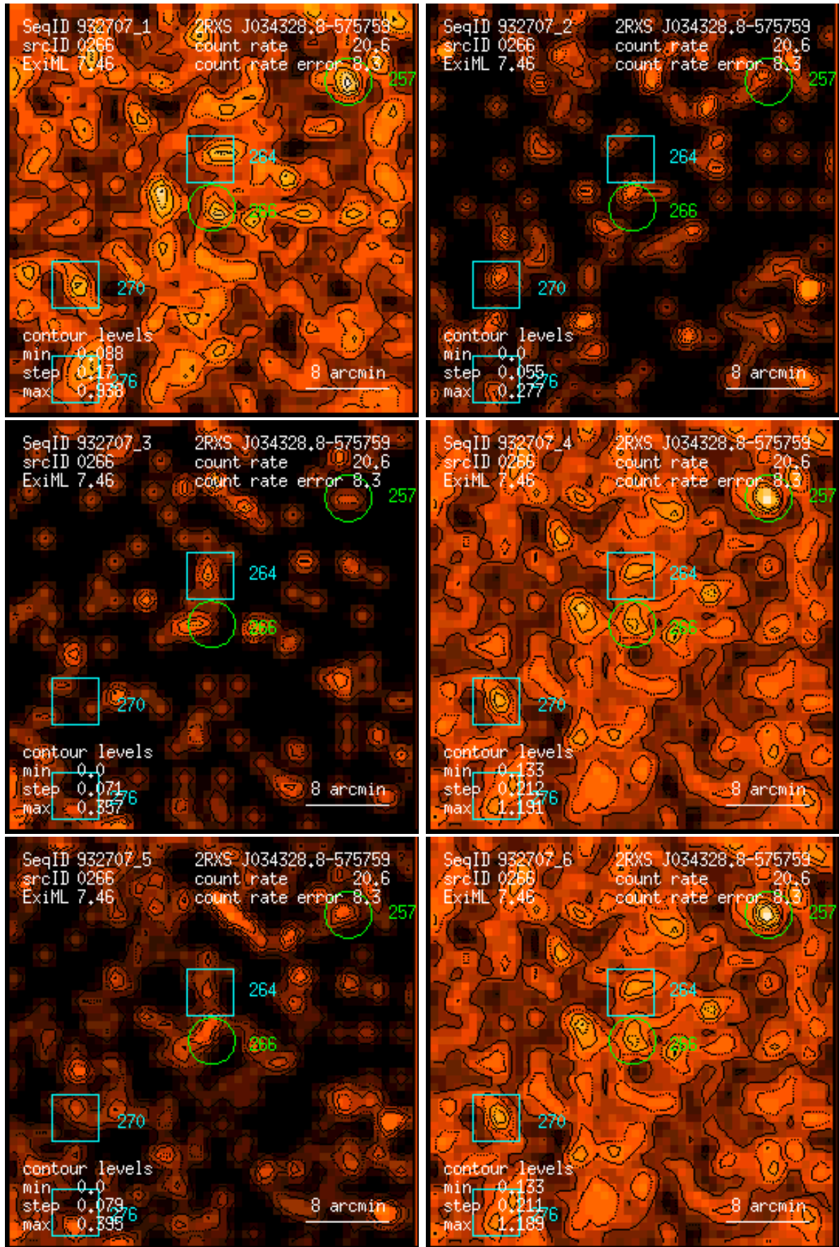
Figure 266: RASS 932707: detection 0266: band rate images, Gaussian filter: (1) PSPC channels 11 – 41, (2) 52 – 90, (3) 91 – 201, (4) 11 – 235, (5) 52 – 201, (6) 11 – 201. Broad band rates in counts/ks. Band rate contour levels in counts/ks/arcmin 2 .
