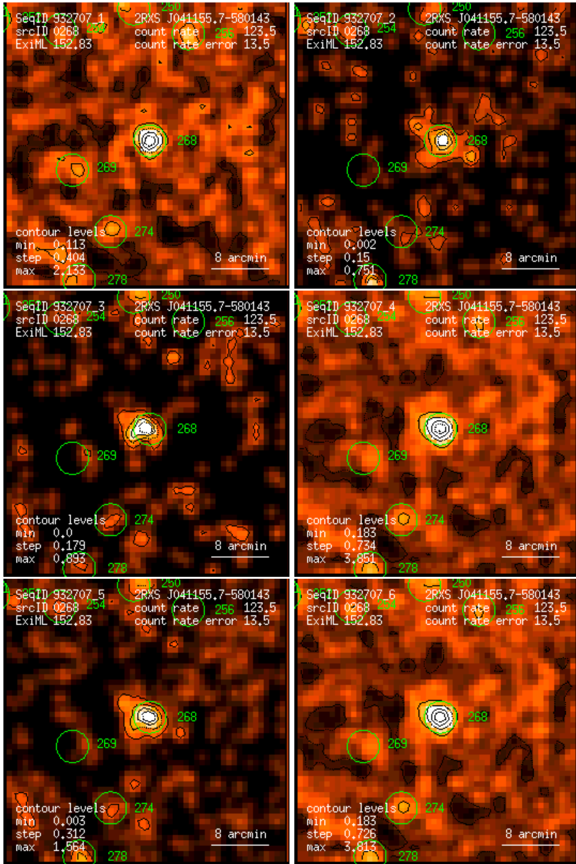
Figure 268: RASS 932707: detection 0268: band rate images, Gaussian filter: (1) PSPC channels 11 – 41, (2) 52 – 90, (3) 91 – 201, (4) 11 – 235, (5) 52 – 201, (6) 11 – 201. Broad band rates in counts/ks. Band rate contour levels in counts/ks/arcmin 2 .
