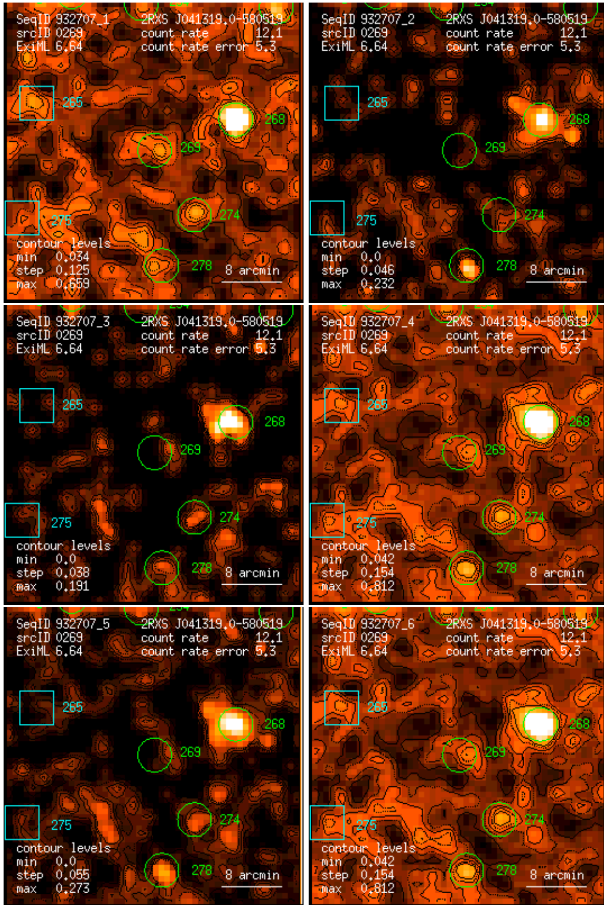
Figure 269: RASS 932707: detection 0269: band rate images, Gaussian filter: (1) PSPC channels 11 – 41, (2) 52 – 90, (3) 91 – 201, (4) 11 – 235, (5) 52 – 201, (6) 11 – 201. Broad band rates in counts/ks. Band rate contour levels in counts/ks/arcmin 2 .
