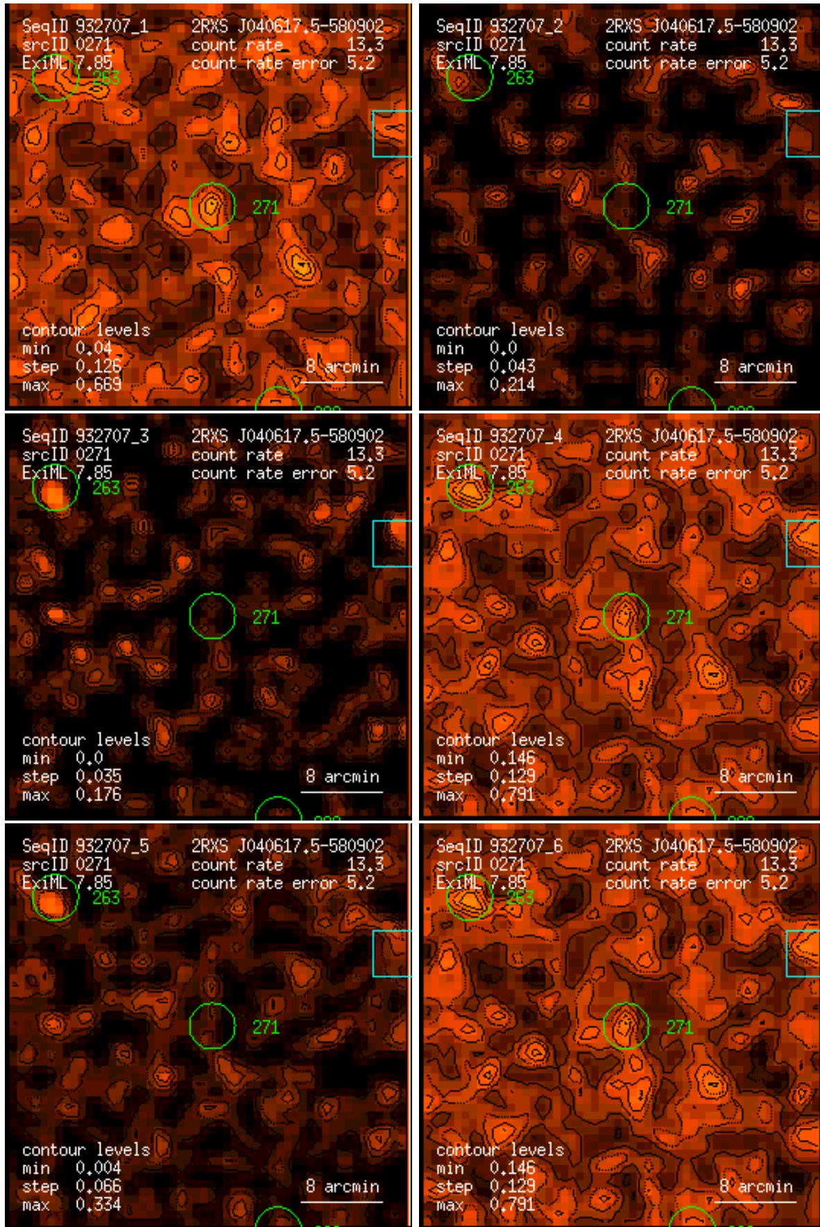
Figure 271: RASS 932707: detection 0271: band rate images, Gaussian filter: (1) PSPC channels 11 – 41, (2) 52 – 90, (3) 91 – 201, (4) 11 – 235, (5) 52 – 201, (6) 11 – 201. Broad band rates in counts/ks. Band rate contour levels in counts/ks/arcmin 2 .
