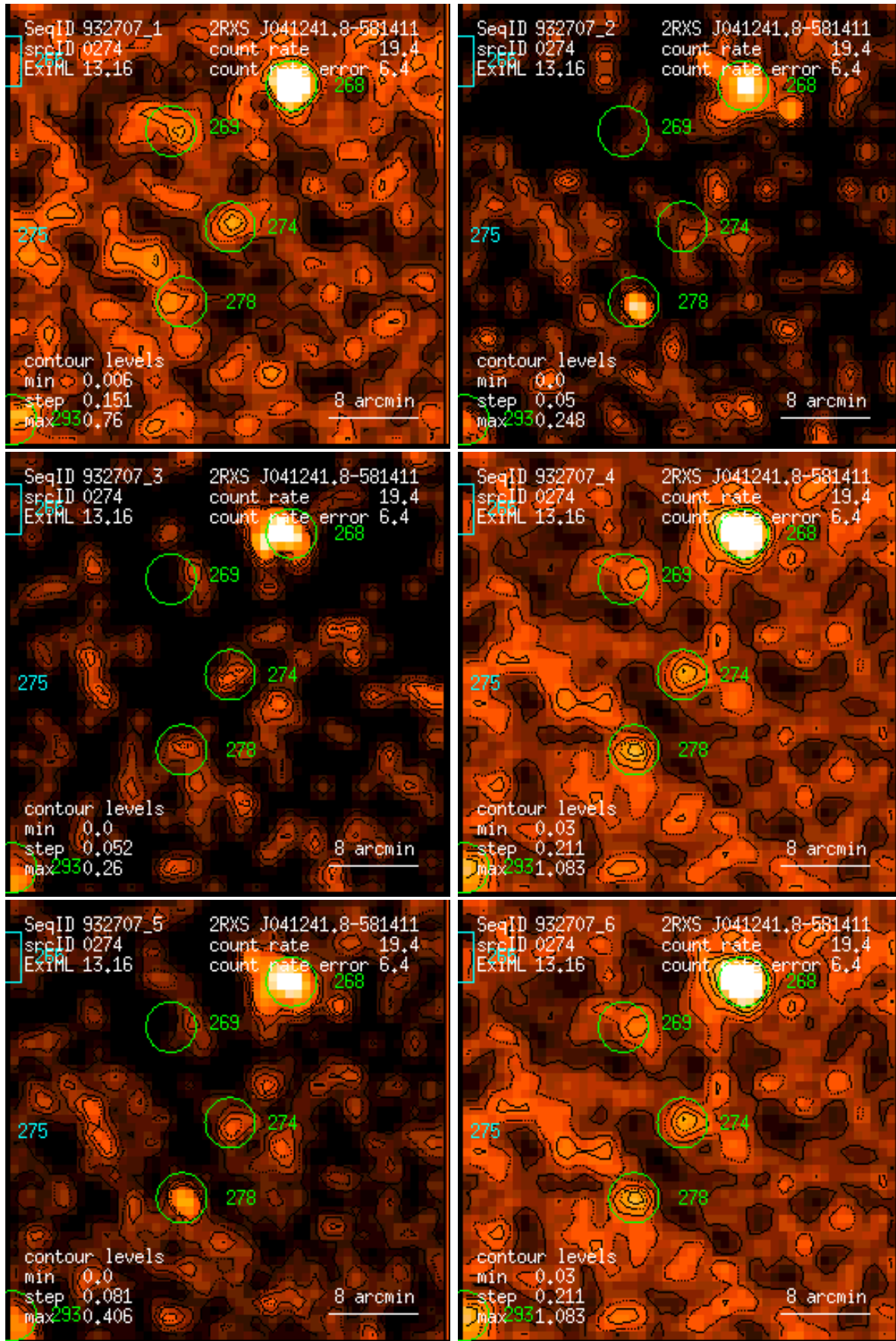
Figure 274: RASS 932707: detection 0274: band rate images, Gaussian filter: (1) PSPC channels 11 – 41, (2) 52 – 90, (3) 91 – 201, (4) 11 – 235, (5) 52 – 201, (6) 11 – 201. Broad band rates in counts/ks. Band rate contour levels in counts/ks/arcmin 2 .
