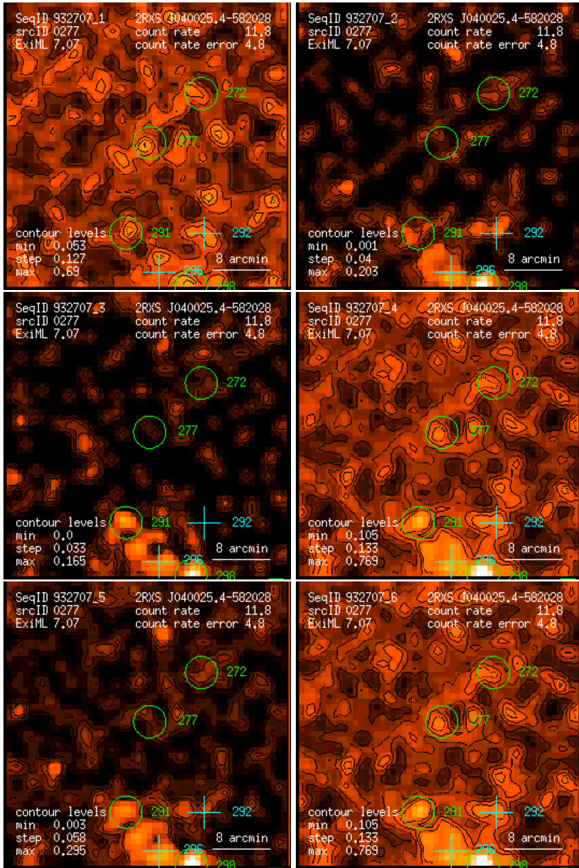
Figure 277: RASS 932707: detection 0277: band rate images, Gaussian filter: (1) PSPC channels 11 – 41, (2) 52 – 90, (3) 91 – 201, (4) 11 – 235, (5) 52 – 201, (6) 11 – 201. Broad band rates in counts/ks. Band rate contour levels in counts/ks/arcmin 2 .
