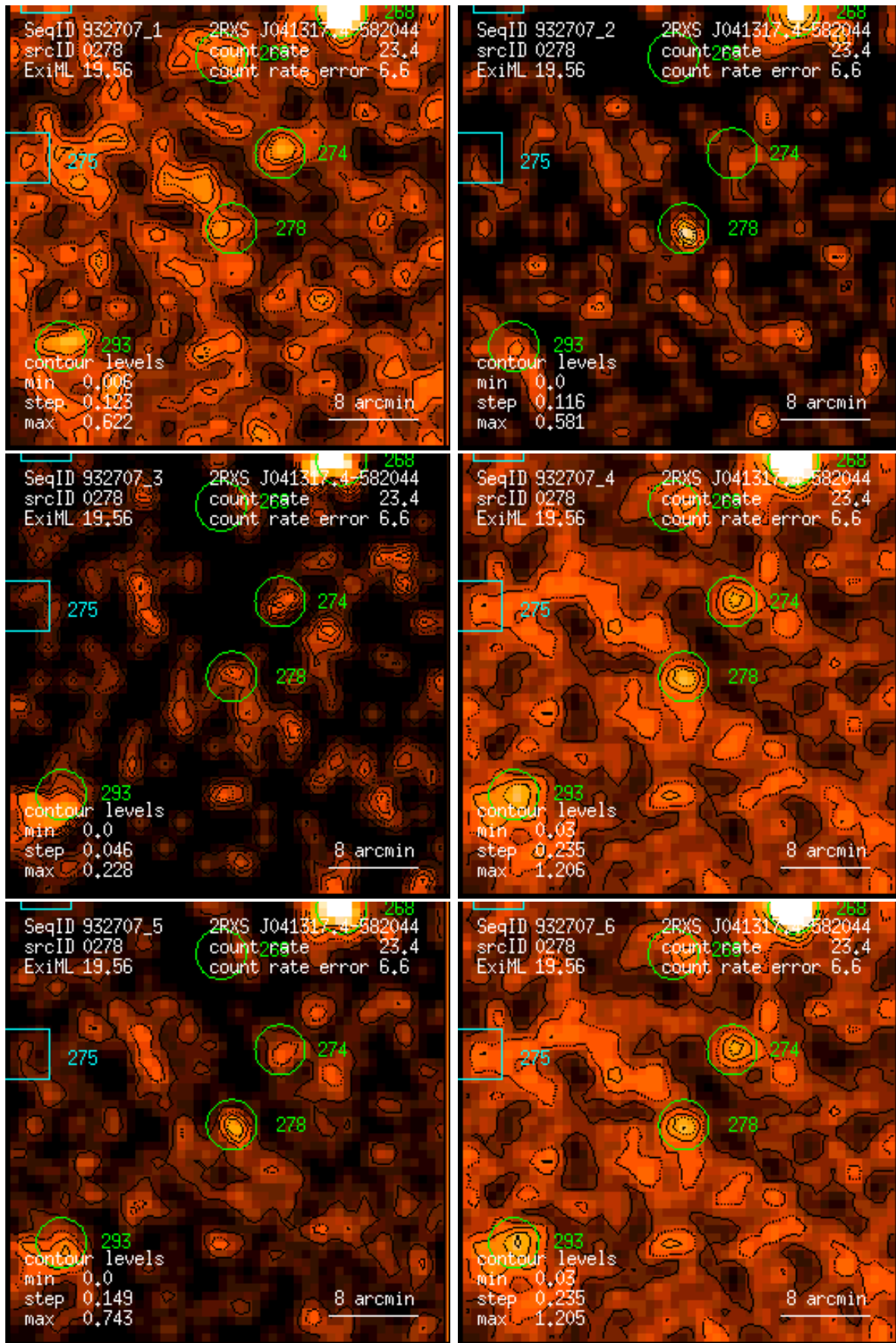
Figure 278: RASS 932707: detection 0278: band rate images, Gaussian filter: (1) PSPC channels 11 – 41, (2) 52 – 90, (3) 91 – 201, (4) 11 – 235, (5) 52 – 201, (6) 11 – 201. Broad band rates in counts/ks. Band rate contour levels in counts/ks/arcmin 2 .
