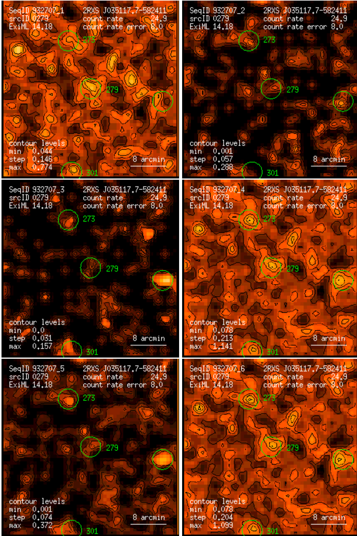
Figure 279: RASS 932707: detection 0279: band rate images, Gaussian filter: (1) PSPC channels 11 – 41, (2) 52 – 90, (3) 91 – 201, (4) 11 – 235, (5) 52 – 201, (6) 11 – 201. Broad band rates in counts/ks. Band rate contour levels in counts/ks/arcmin 2 .
