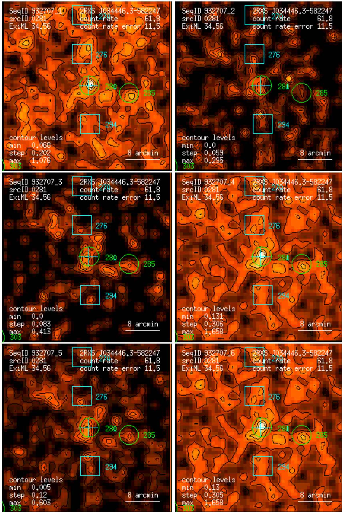
Figure 281: RASS 932707: detection 0281: band rate images, Gaussian filter: (1) PSPC channels 11 – 41, (2) 52 – 90, (3) 91 – 201, (4) 11 – 235, (5) 52 – 201, (6) 11 – 201. Broad band rates in counts/ks. Band rate contour levels in counts/ks/arcmin 2 .
