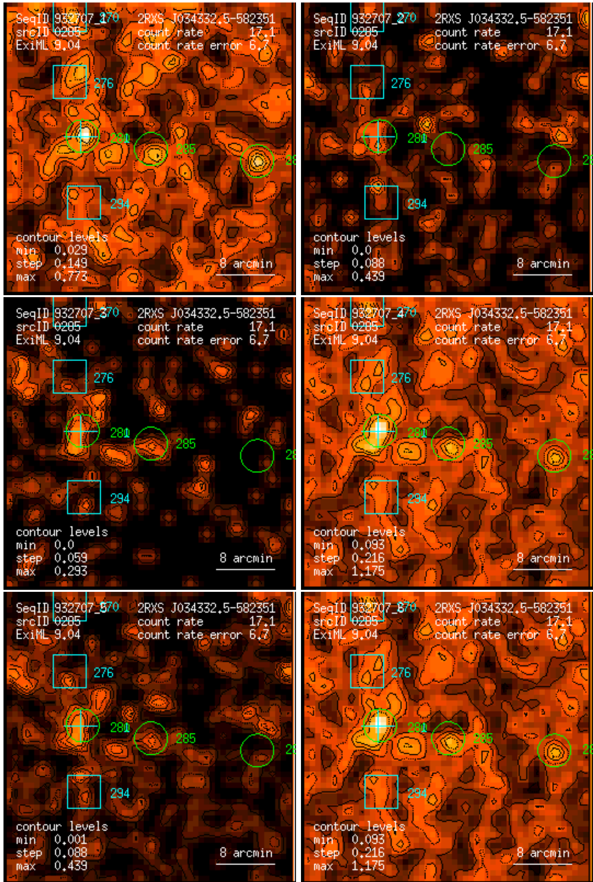
Figure 285: RASS 932707: detection 0285: band rate images, Gaussian filter: (1) PSPC channels 11 – 41, (2) 52 – 90, (3) 91 – 201, (4) 11 – 235, (5) 52 – 201, (6) 11 – 201. Broad band rates in counts/ks. Band rate contour levels in counts/ks/arcmin 2 .
