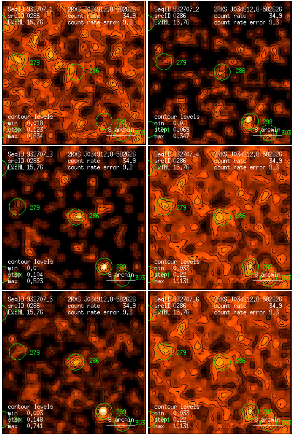
Figure 286: RASS 932707: detection 0286: band rate images, Gaussian filter: (1) PSPC channels 11 – 41, (2) 52 – 90, (3) 91 – 201, (4) 11 – 235, (5) 52 – 201, (6) 11 – 201. Broad band rates in counts/ks. Band rate contour levels in counts/ks/arcmin 2 .
