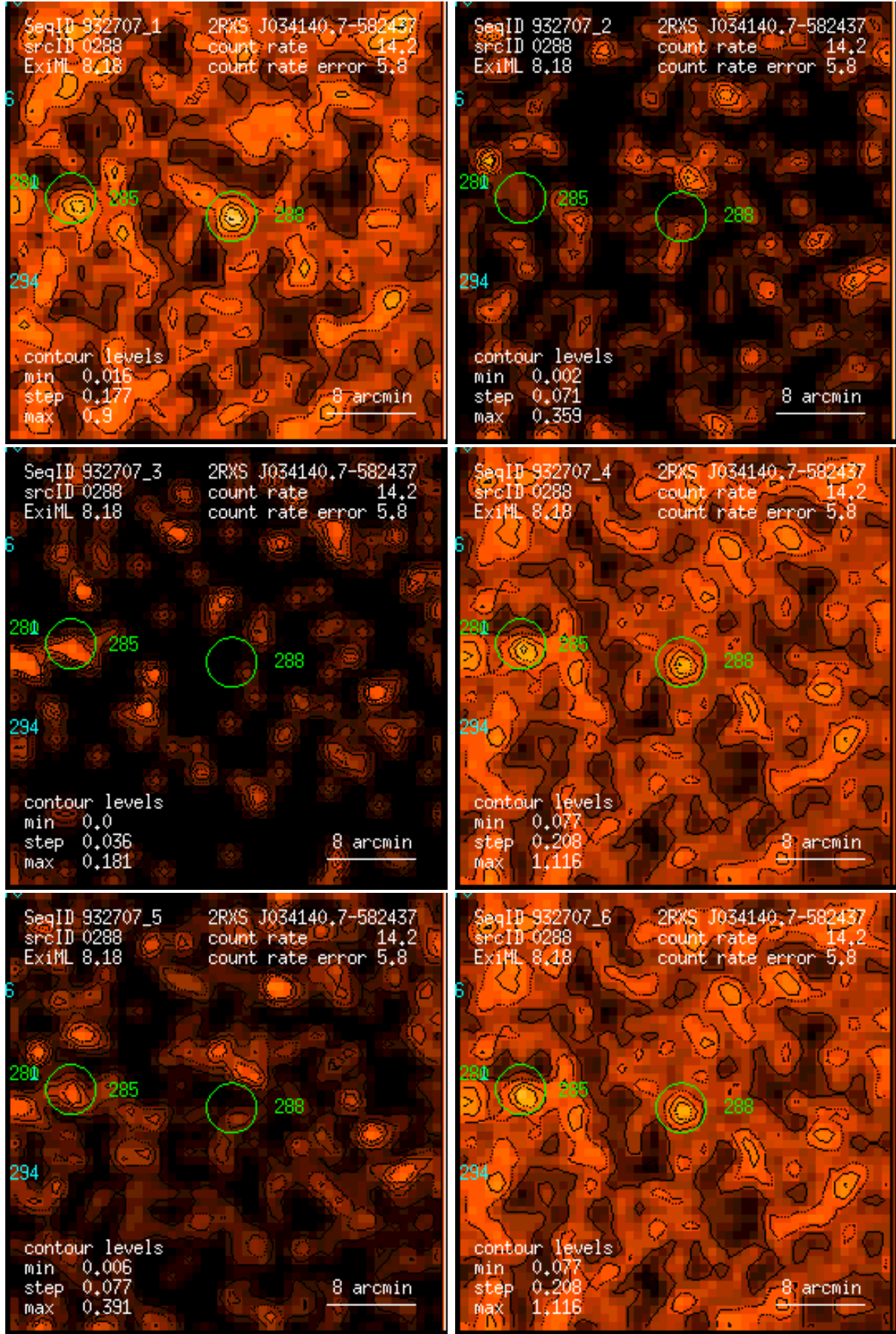
Figure 288: RASS 932707: detection 0288: band rate images, Gaussian filter: (1) PSPC channels 11 – 41, (2) 52 – 90, (3) 91 – 201, (4) 11 – 235, (5) 52 – 201, (6) 11 – 201. Broad band rates in counts/ks. Band rate contour levels in counts/ks/arcmin 2 .
