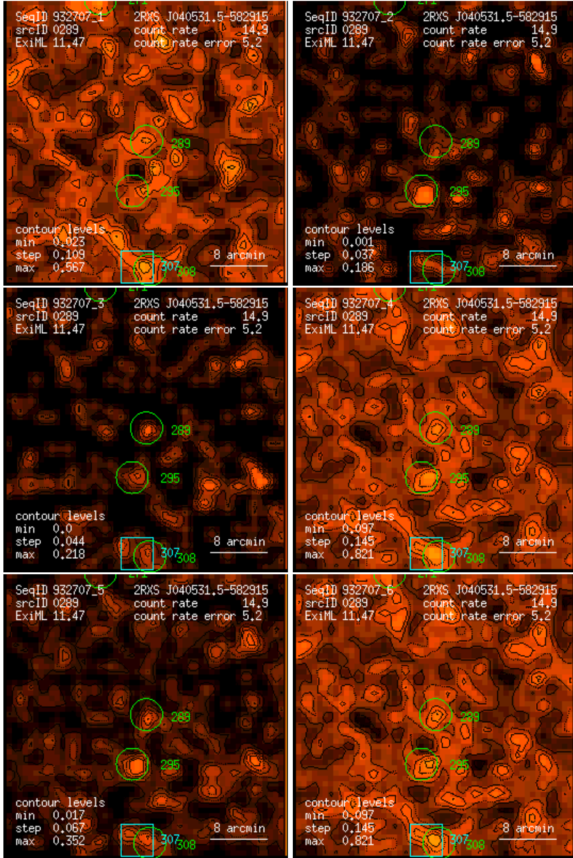
Figure 289: RASS 932707: detection 0289: band rate images, Gaussian filter: (1) PSPC channels 11 – 41, (2) 52 – 90, (3) 91 – 201, (4) 11 – 235, (5) 52 – 201, (6) 11 – 201. Broad band rates in counts/ks. Band rate contour levels in counts/ks/arcmin 2 .
