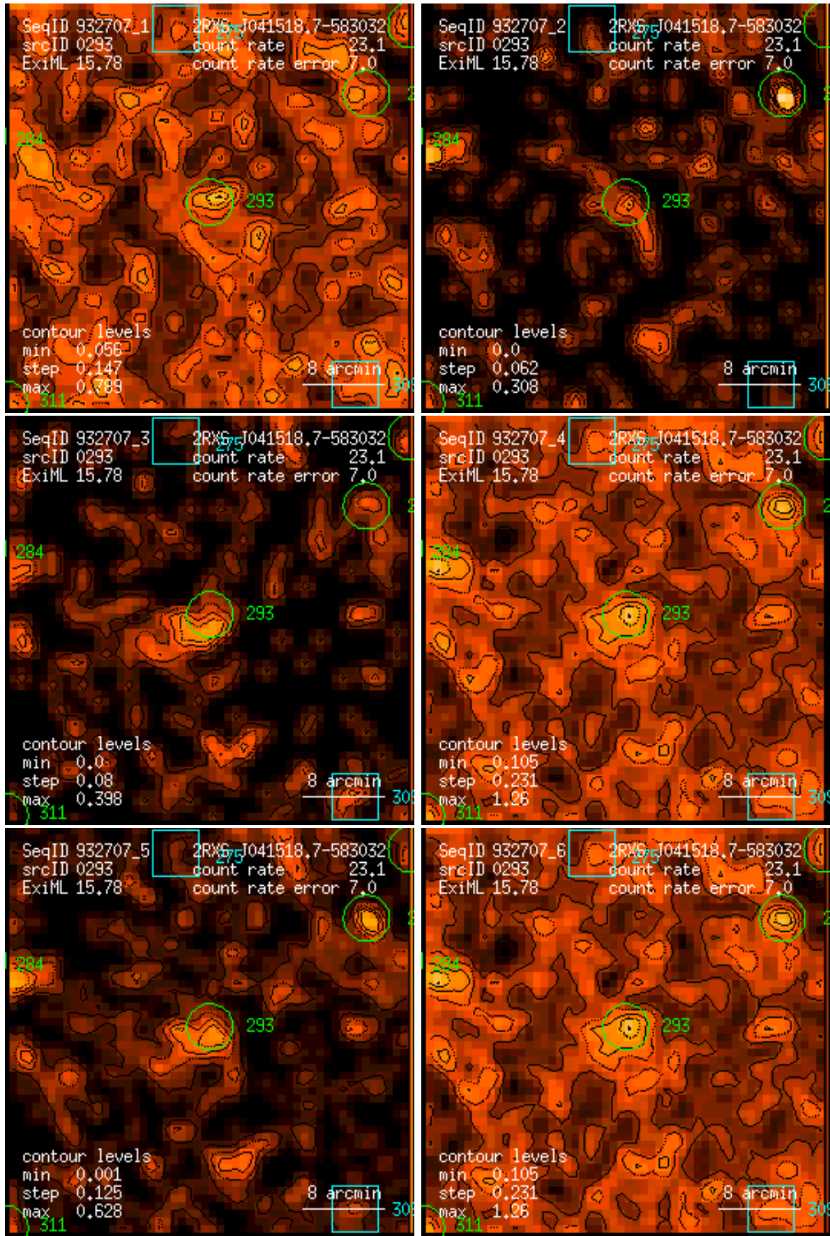
Figure 293: RASS 932707: detection 0293: band rate images, Gaussian filter: (1) PSPC channels 11 – 41, (2) 52 – 90, (3) 91 – 201, (4) 11 – 235, (5) 52 – 201, (6) 11 – 201. Broad band rates in counts/ks. Band rate contour levels in counts/ks/arcmin 2 .
