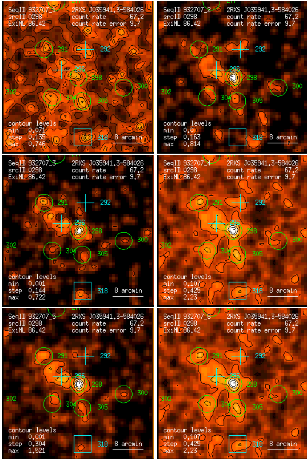
Figure 298: RASS 932707: detection 0298: band rate images, Gaussian filter: (1) PSPC channels 11 – 41, (2) 52 – 90, (3) 91 – 201, (4) 11 – 235, (5) 52 – 201, (6) 11 – 201. Broad band rates in counts/ks. Band rate contour levels in counts/ks/arcmin 2 .
