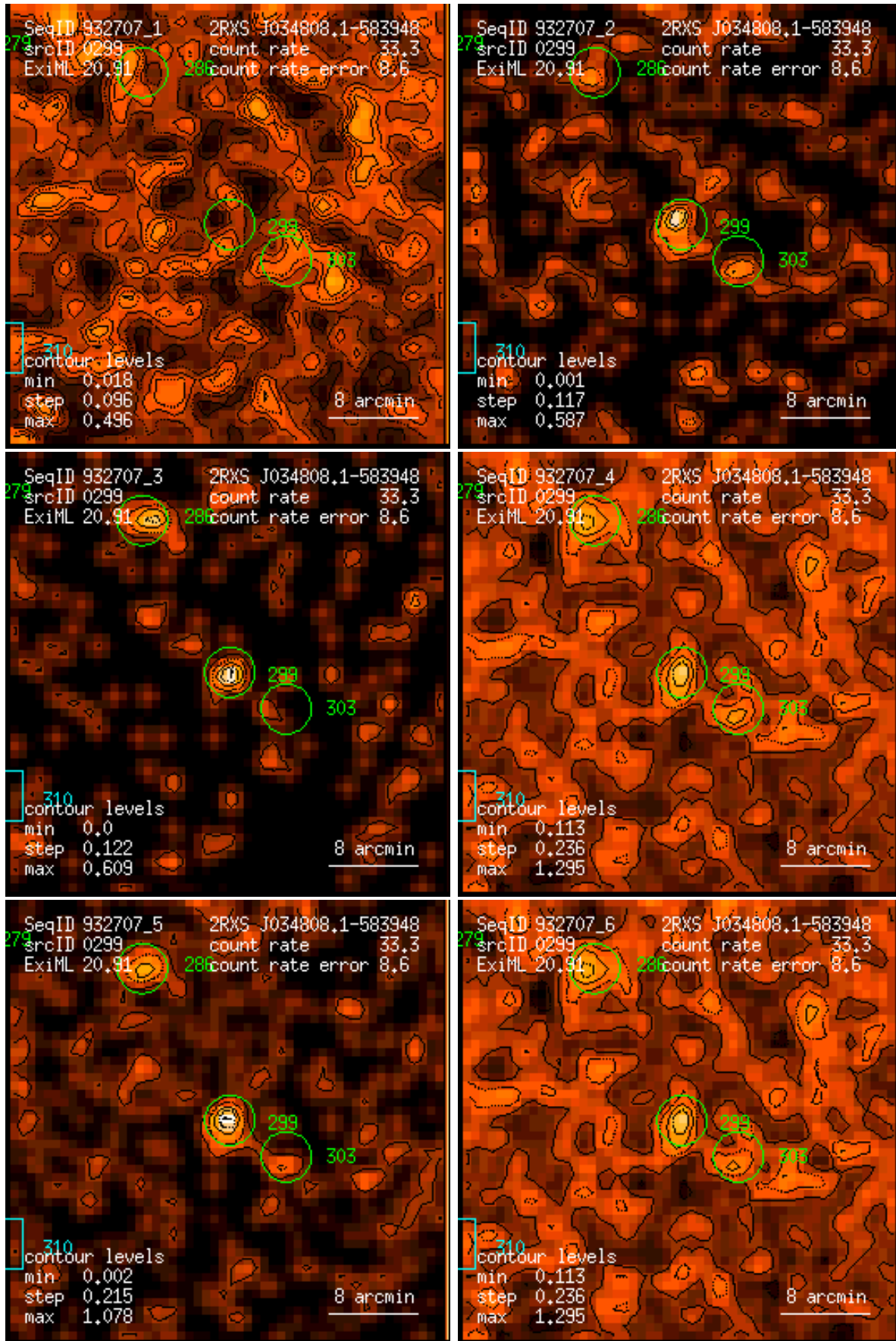
Figure 299: RASS 932707: detection 0299: band rate images, Gaussian filter: (1) PSPC channels 11 – 41, (2) 52 – 90, (3) 91 – 201, (4) 11 – 235, (5) 52 – 201, (6) 11 – 201. Broad band rates in counts/ks. Band rate contour levels in counts/ks/arcmin 2 .
