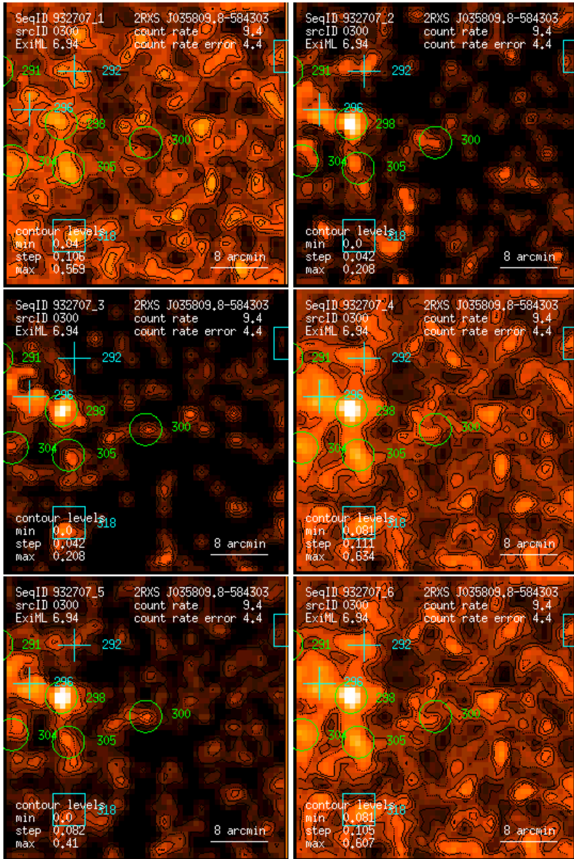
Figure 300: RASS 932707: detection 0300: band rate images, Gaussian filter: (1) PSPC channels 11 – 41, (2) 52 – 90, (3) 91 – 201, (4) 11 – 235, (5) 52 – 201, (6) 11 – 201. Broad band rates in counts/ks. Band rate contour levels in counts/ks/arcmin 2 .
