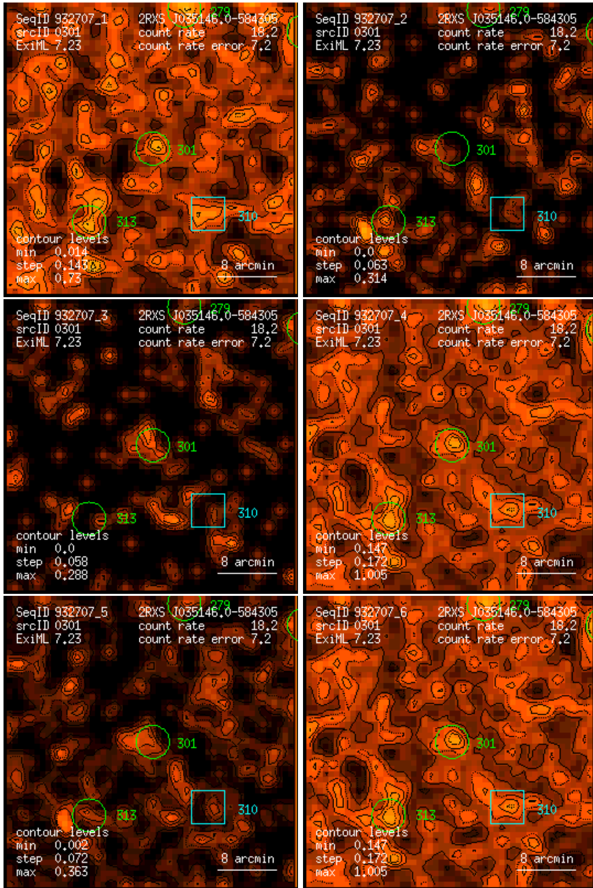
Figure 301: RASS 932707: detection 0301: band rate images, Gaussian filter: (1) PSPC channels 11 – 41, (2) 52 – 90, (3) 91 – 201, (4) 11 – 235, (5) 52 – 201, (6) 11 – 201. Broad band rates in counts/ks. Band rate contour levels in counts/ks/arcmin 2 .
