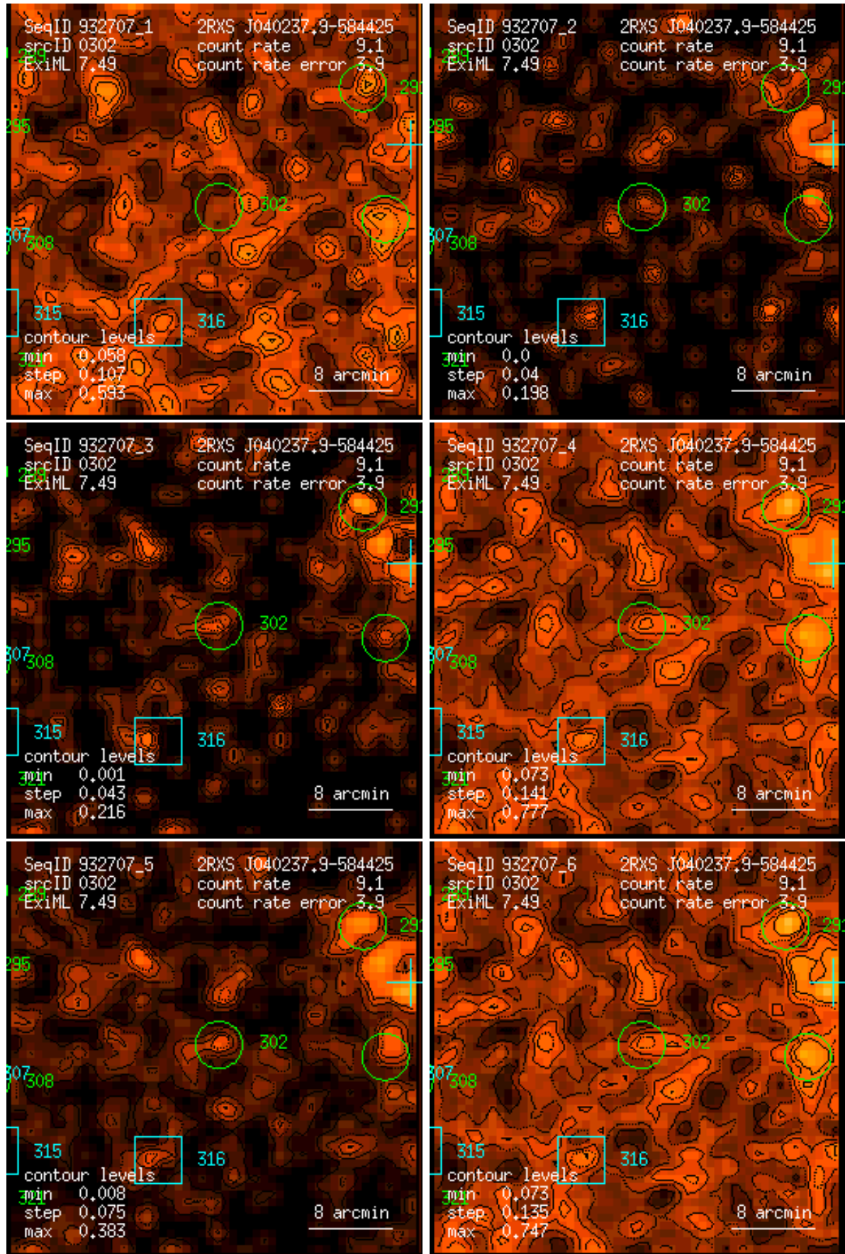
Figure 302: RASS 932707: detection 0302: band rate images, Gaussian filter: (1) PSPC channels 11 – 41, (2) 52 – 90, (3) 91 – 201, (4) 11 – 235, (5) 52 – 201, (6) 11 – 201. Broad band rates in counts/ks. Band rate contour levels in counts/ks/arcmin 2 .
