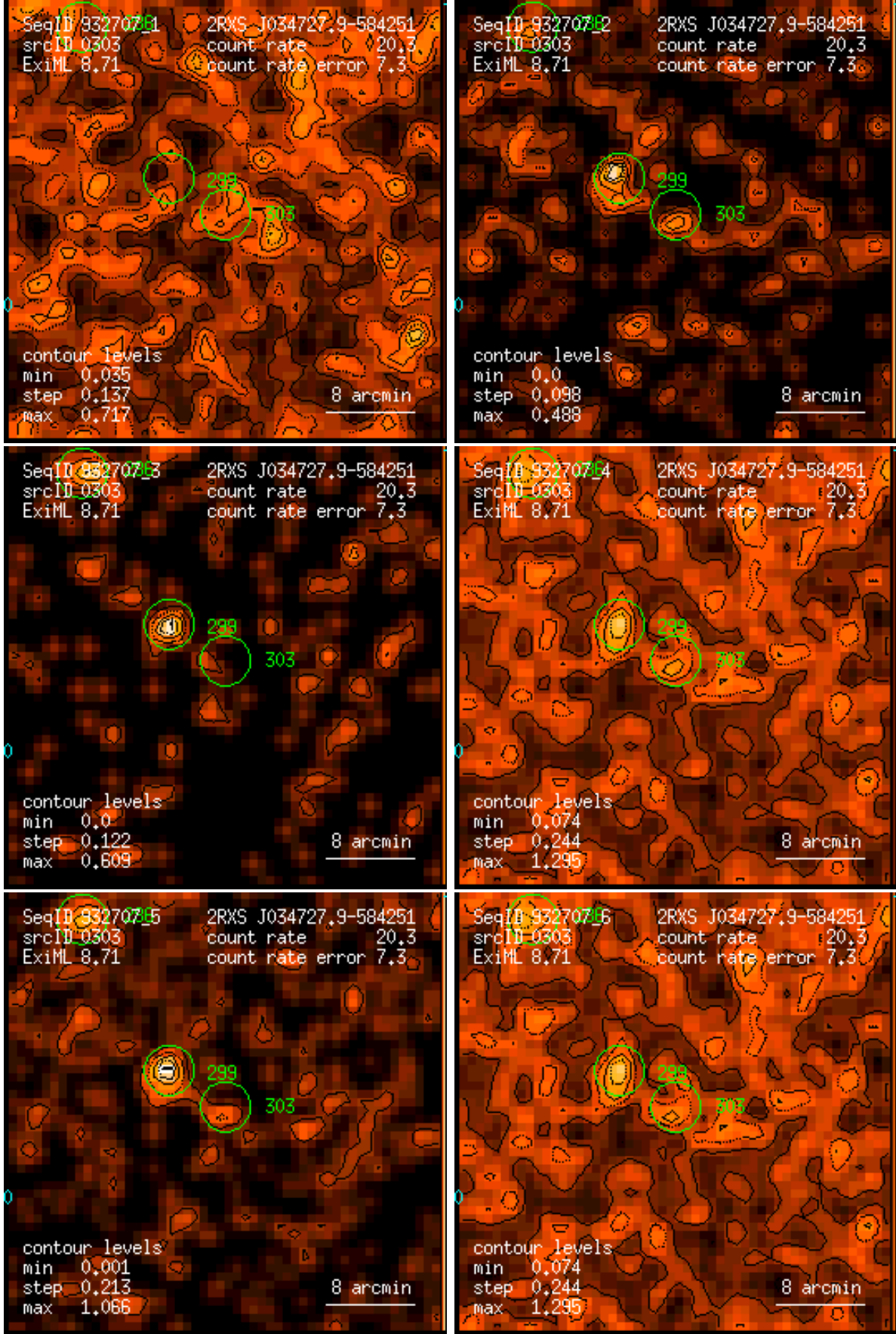
Figure 303: RASS 932707: detection 0303: band rate images, Gaussian filter: (1) PSPC channels 11 – 41, (2) 52 – 90, (3) 91 – 201, (4) 11 – 235, (5) 52 – 201, (6) 11 – 201. Broad band rates in counts/ks. Band rate contour levels in counts/ks/arcmin 2 .
