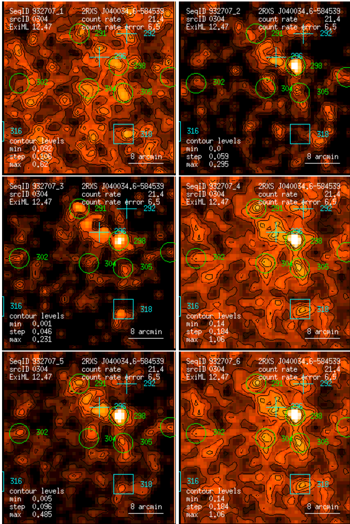
Figure 304: RASS 932707: detection 0304: band rate images, Gaussian filter: (1) PSPC channels 11 – 41, (2) 52 – 90, (3) 91 – 201, (4) 11 – 235, (5) 52 – 201, (6) 11 – 201. Broad band rates in counts/ks. Band rate contour levels in counts/ks/arcmin 2 .
