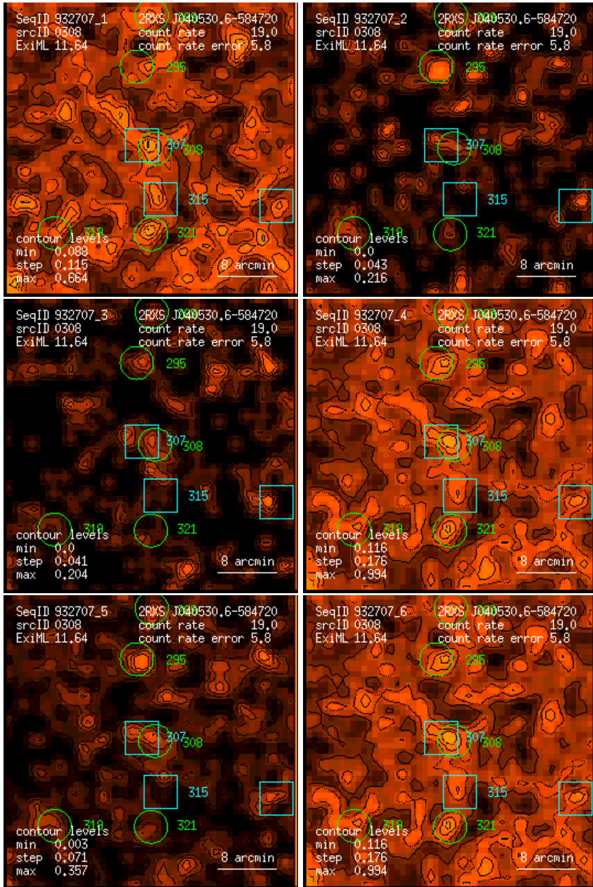
Figure 308: RASS 932707: detection 0308: band rate images, Gaussian filter: (1) PSPC channels 11 – 41, (2) 52 – 90, (3) 91 – 201, (4) 11 – 235, (5) 52 – 201, (6) 11 – 201. Broad band rates in counts/ks. Band rate contour levels in counts/ks/arcmin 2 .
