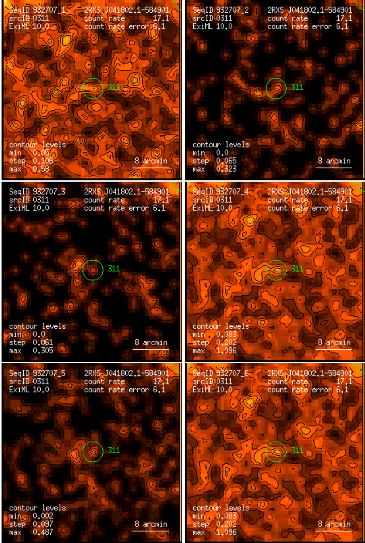
Figure 311: RASS 932707: detection 0311: band rate images, Gaussian filter: (1) PSPC channels 11 – 41, (2) 52 – 90, (3) 91 – 201, (4) 11 – 235, (5) 52 – 201, (6) 11 – 201. Broad band rates in counts/ks. Band rate contour levels in counts/ks/arcmin 2 .
