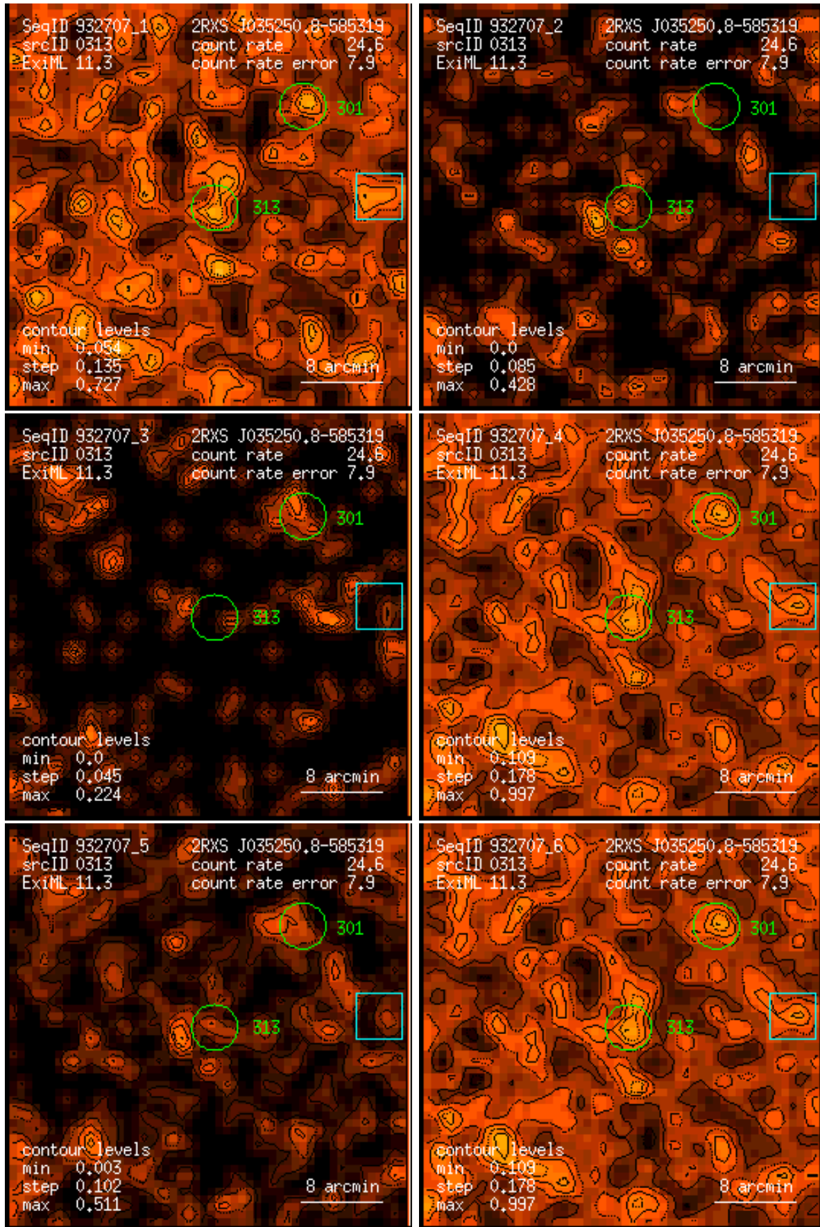
Figure 313: RASS 932707: detection 0313: band rate images, Gaussian filter: (1) PSPC channels 11 – 41, (2) 52 – 90, (3) 91 – 201, (4) 11 – 235, (5) 52 – 201, (6) 11 – 201. Broad band rates in counts/ks. Band rate contour levels in counts/ks/arcmin 2 .
